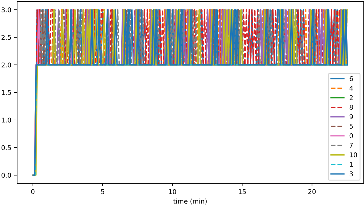
vmap_queries_readEntities_accounts
