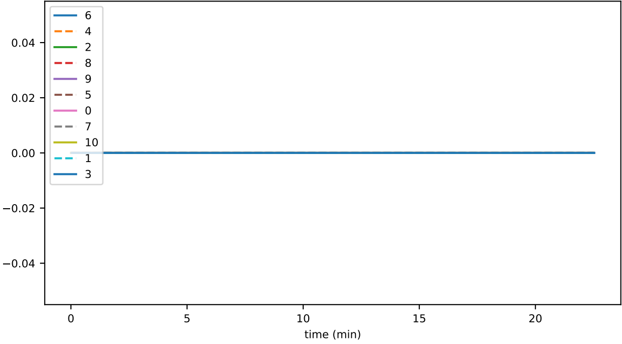
ds_files_level_5_leafKeysFileSizeByLevelMb_accounts
