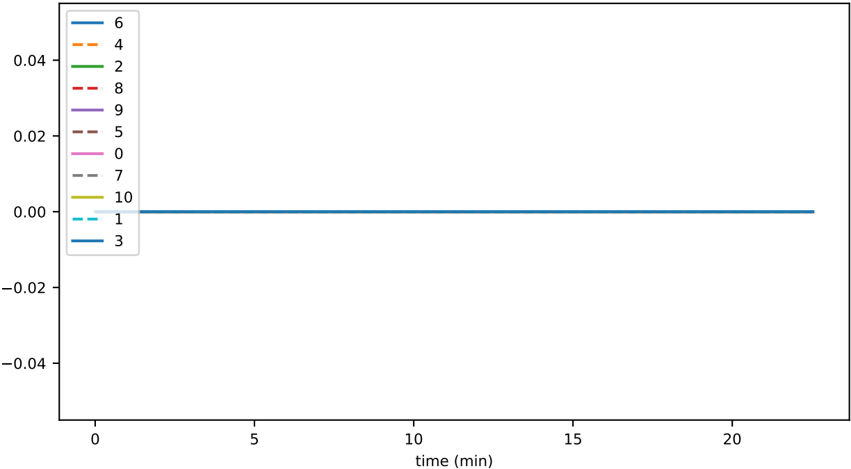
ds_files_level_2_leavesFileSizeByLevelMb_accounts
