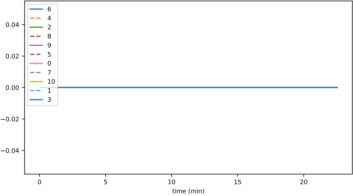
ds_compactions_level_0_leafKeysSavedSpaceMb_accounts
