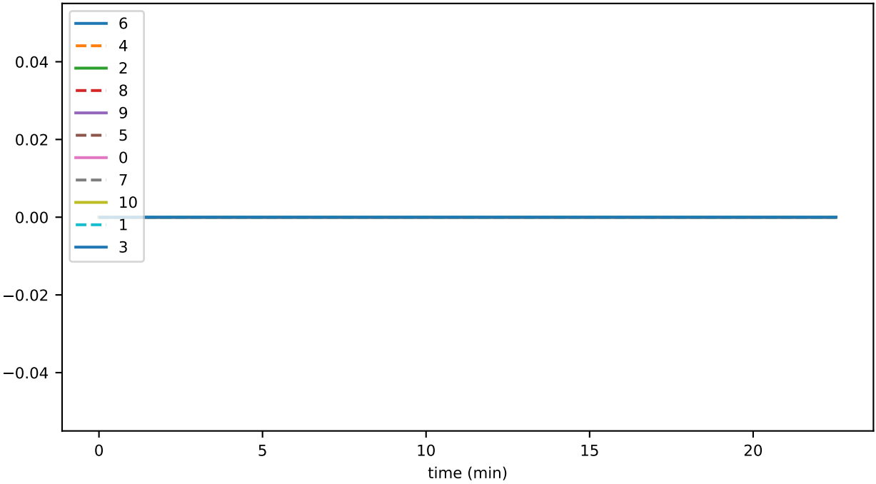
ds_files_level_5_leavesFileSizeByLevelMb_accounts
