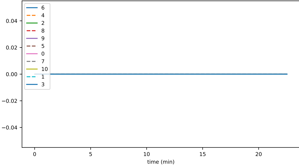
vmap_queries_removedEntities_accounts
