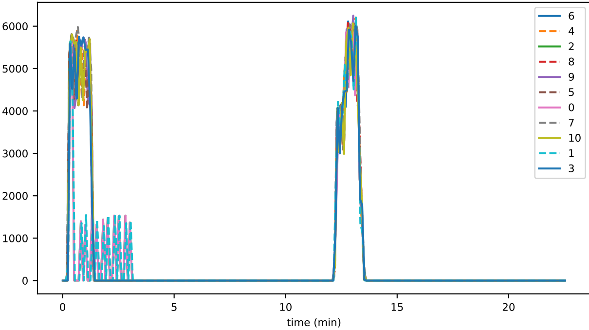
vmap_queries_removedEntities_accounts
