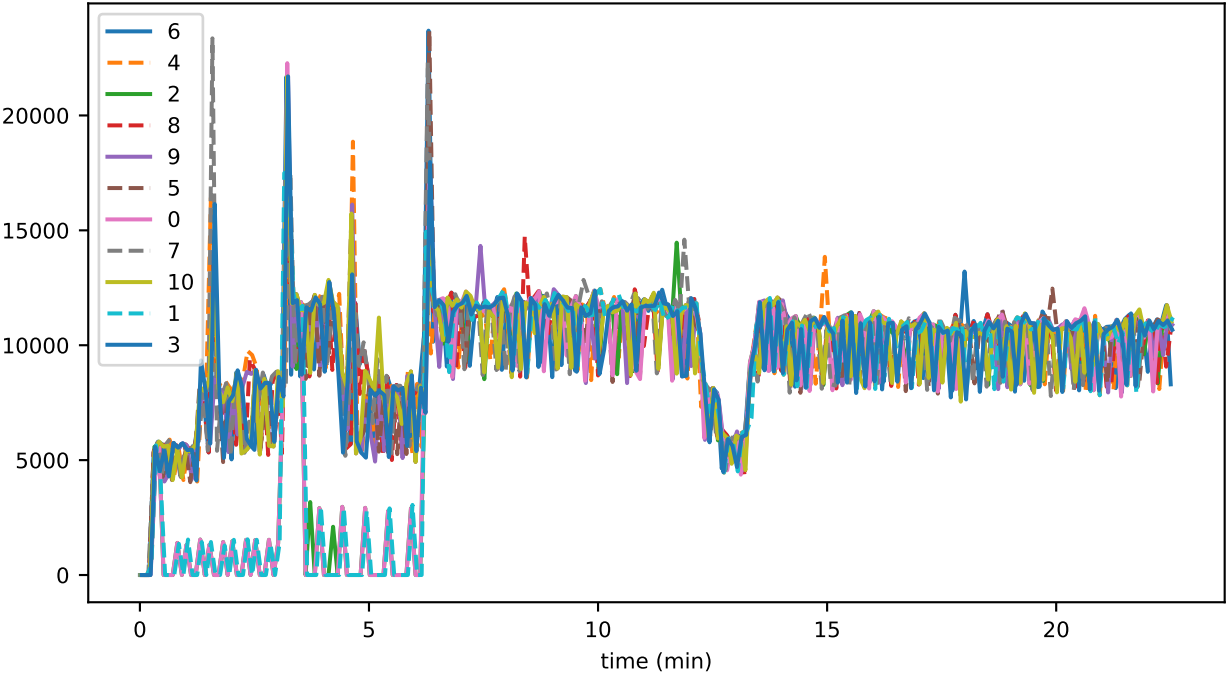
vmap_queries_readEntities_accounts
