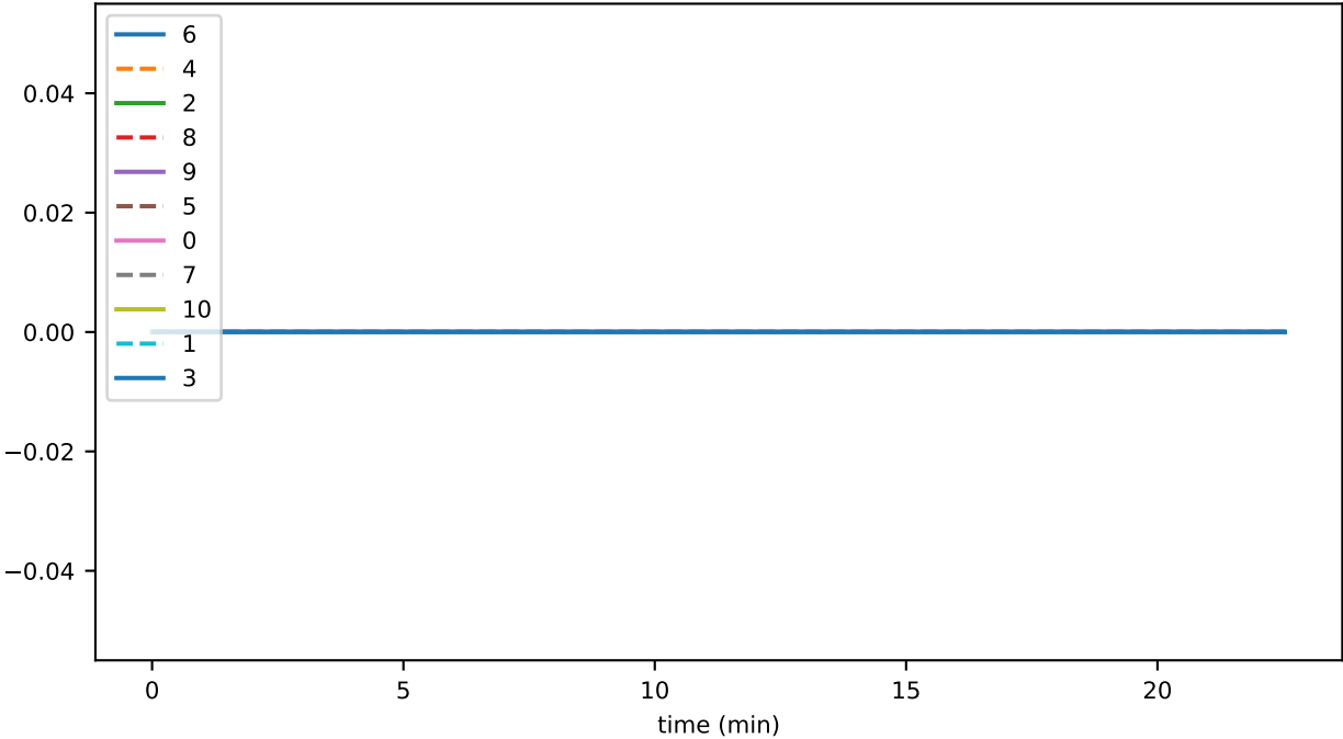
ds_files_level_3_hashesFileSizeByLevelMb_accounts
