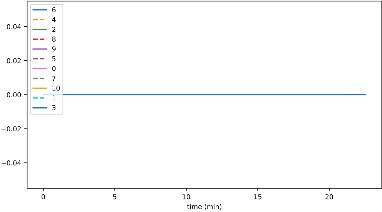
ds_compactions_level_0_leafKeysTimeMs_accounts
