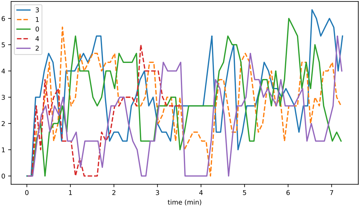
InlinePcesWriter_busy_fraction
