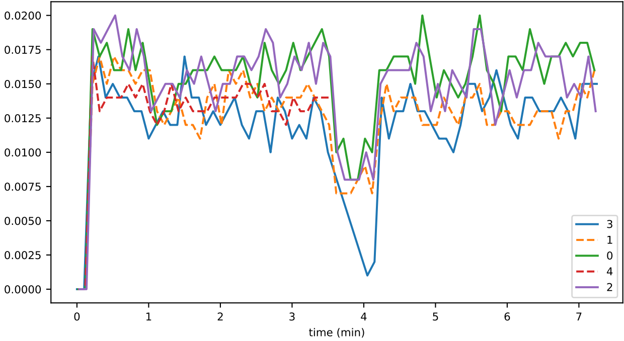
InlinePcesWriter_busy_fraction
