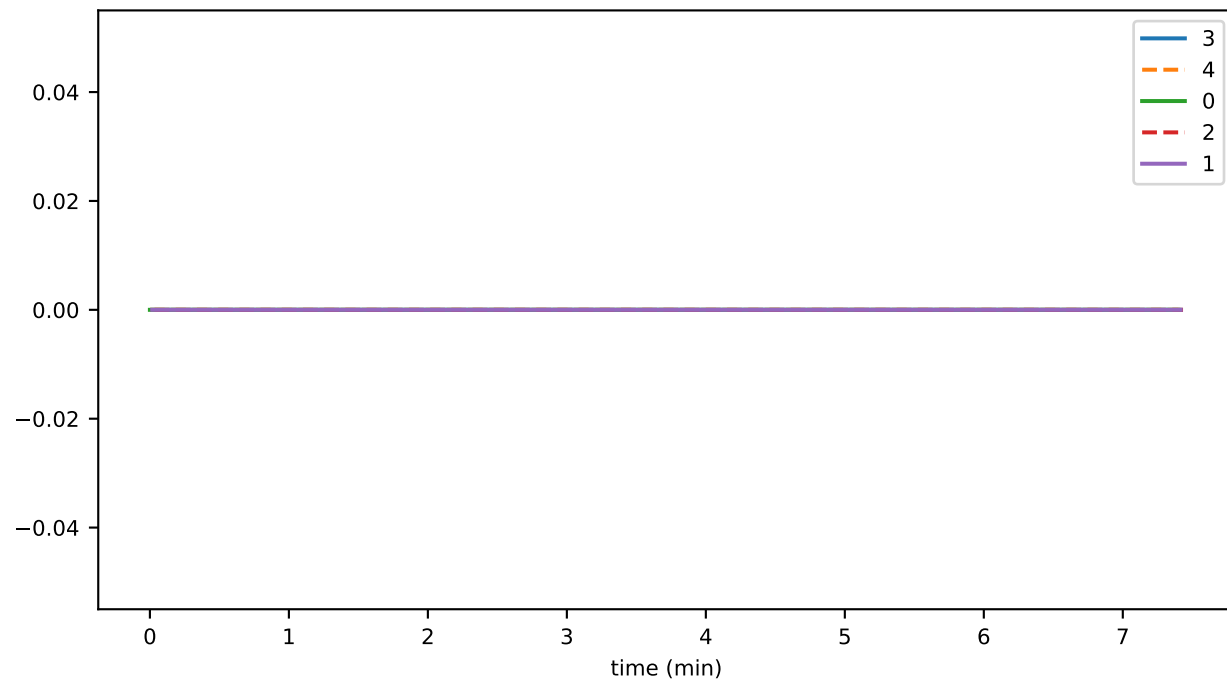
countInMemoryTestMerkleStateRoot
