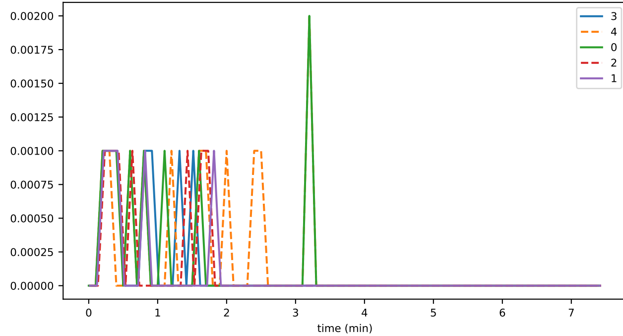
consensus_fraction_SETTING_EVENT_CONSENSUS_DATA
