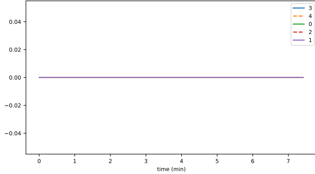
SigIntakePulse_per_sec
