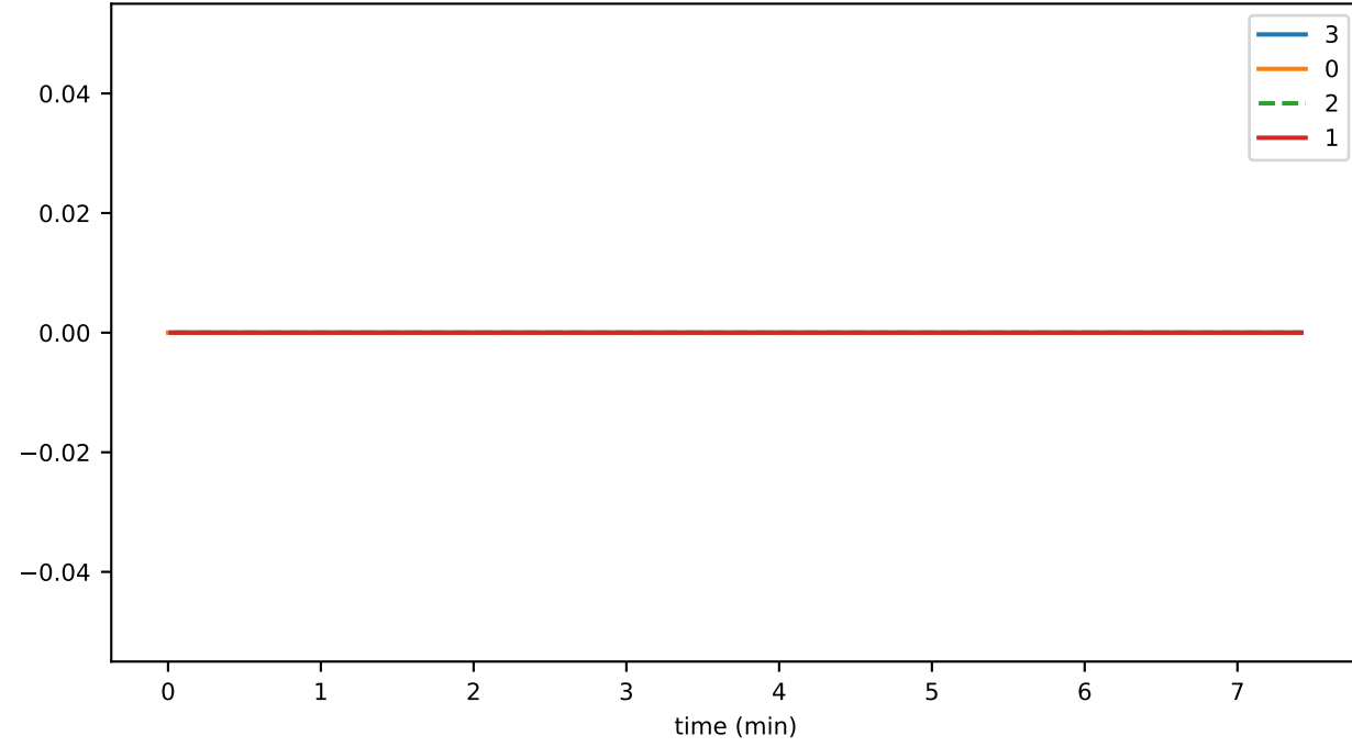
reconnectRejections_per_sec_04
