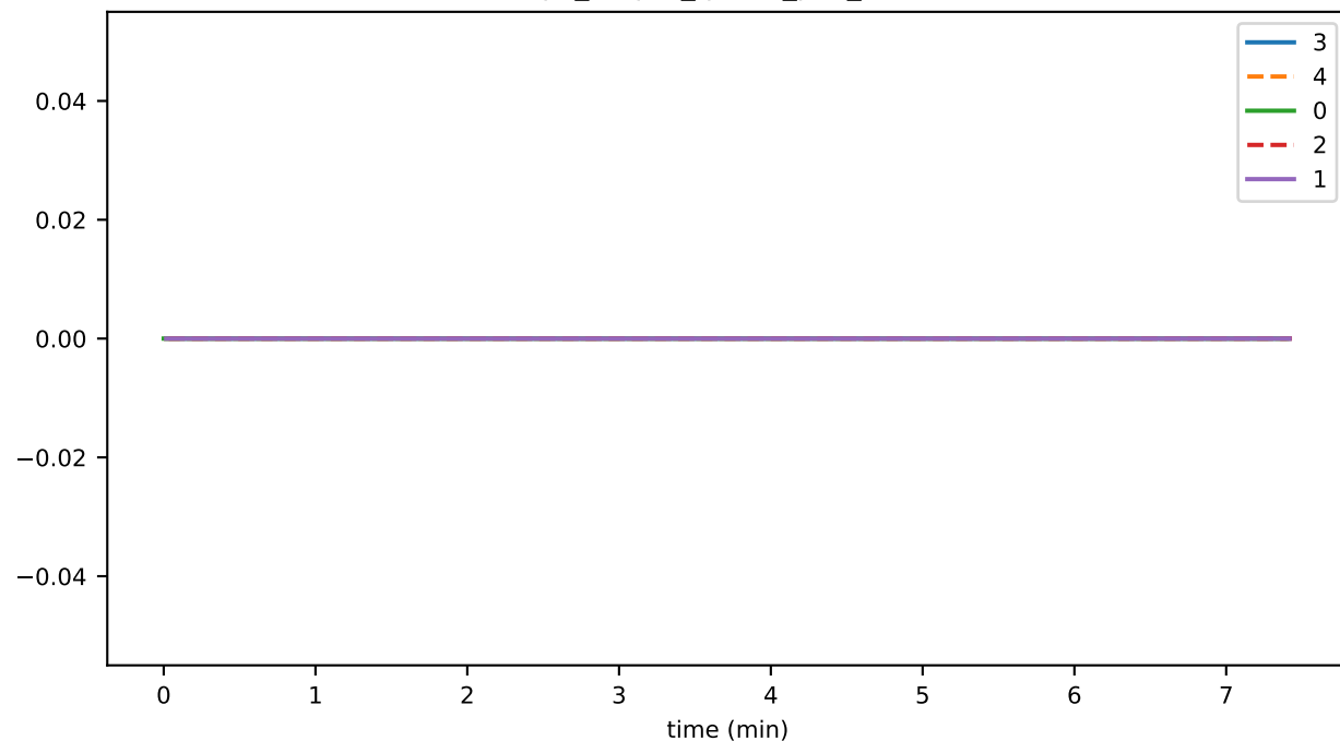
rpcDispatchThreadRunning
