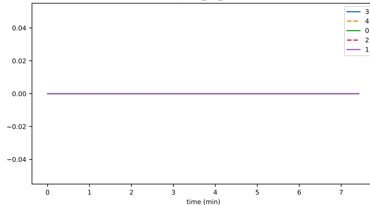
SignedStateSentinel_unhandled_task_count
