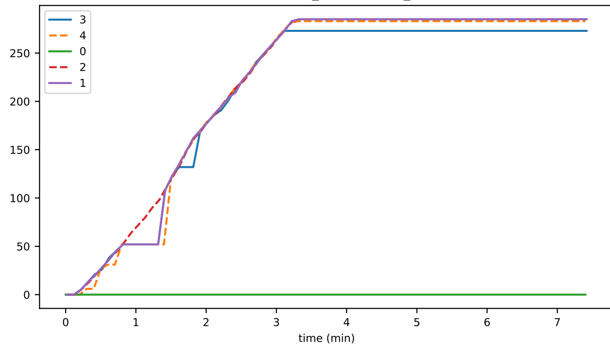
hasFallenBehind
