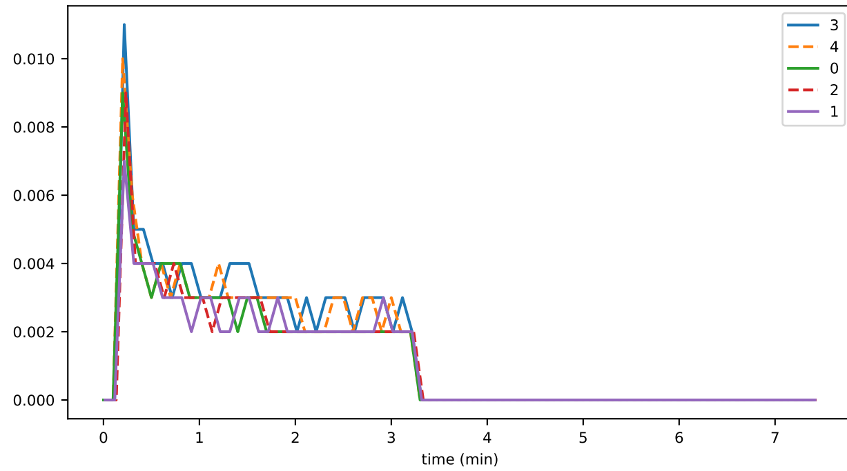
ConsensusEngine_busy_fraction
