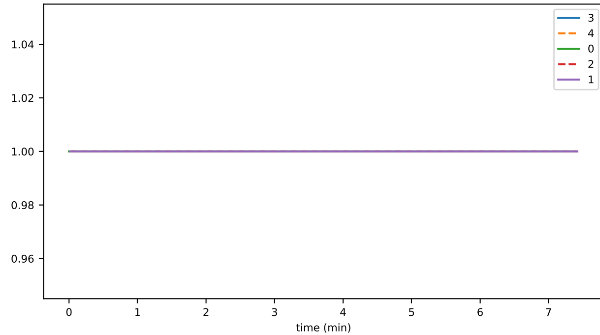
healthy
