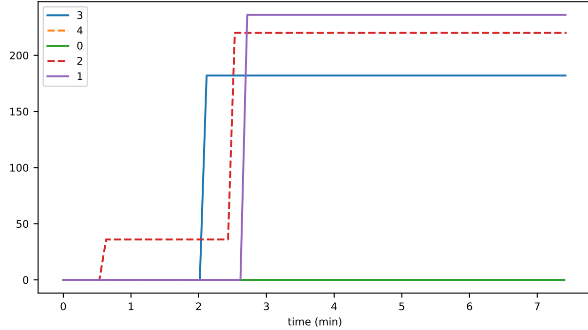
futureEventBuffer_consensus_maxBR
