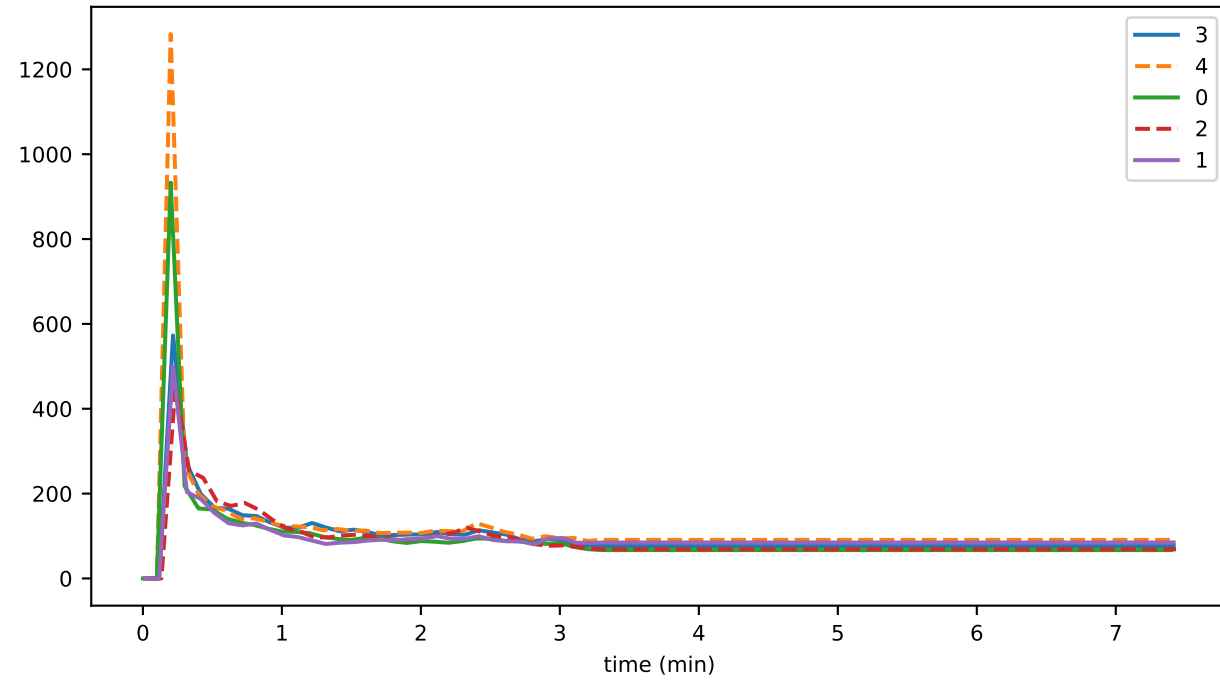
witnessesSeenMAX
