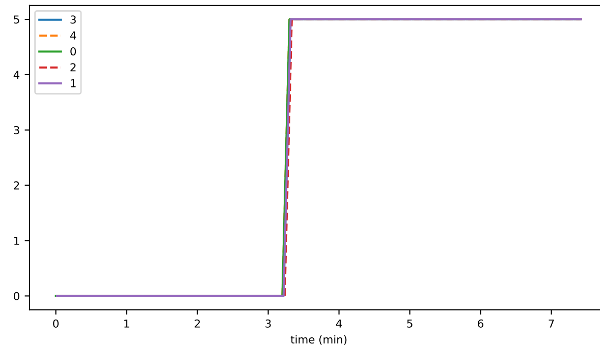
issWeight
