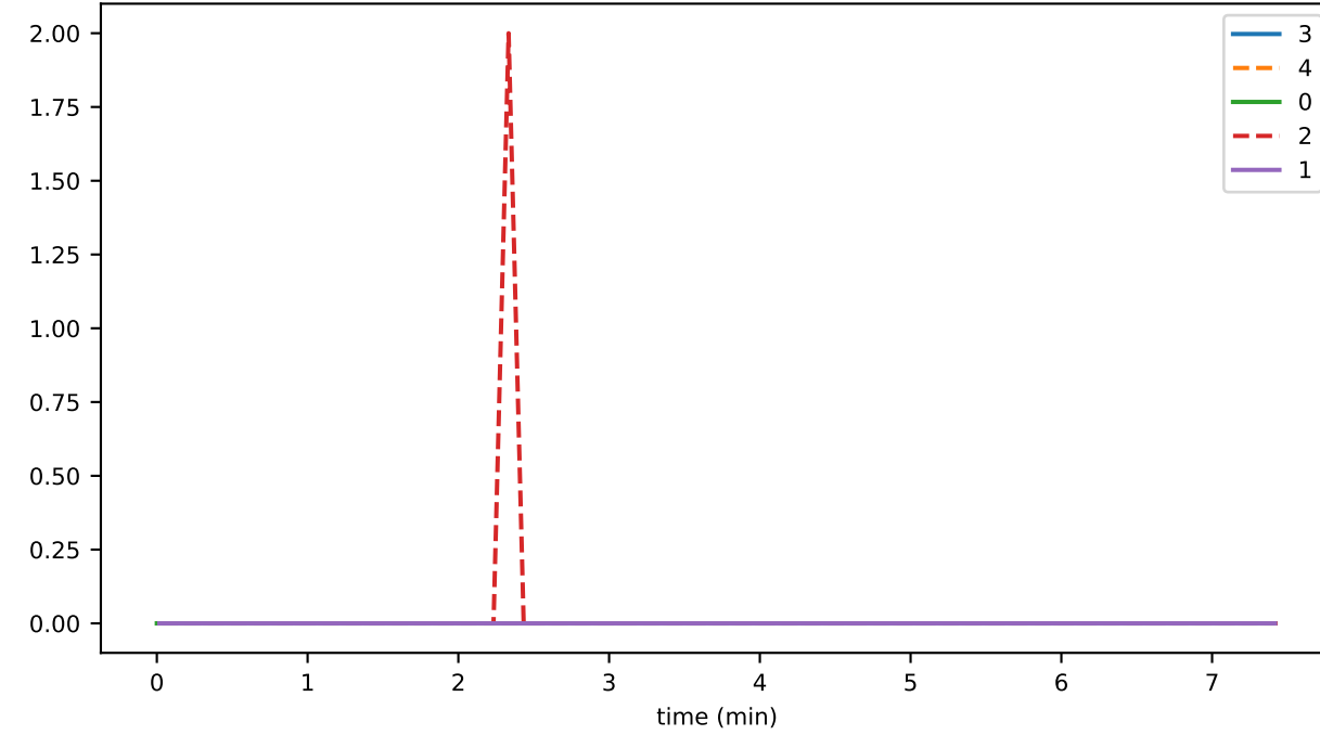
futureEventBuffer_eventCreator_count
