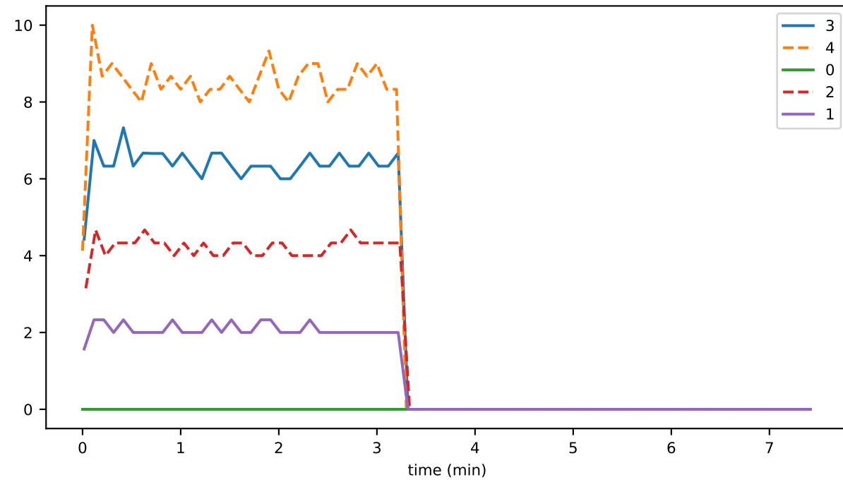
sync_per_secR
