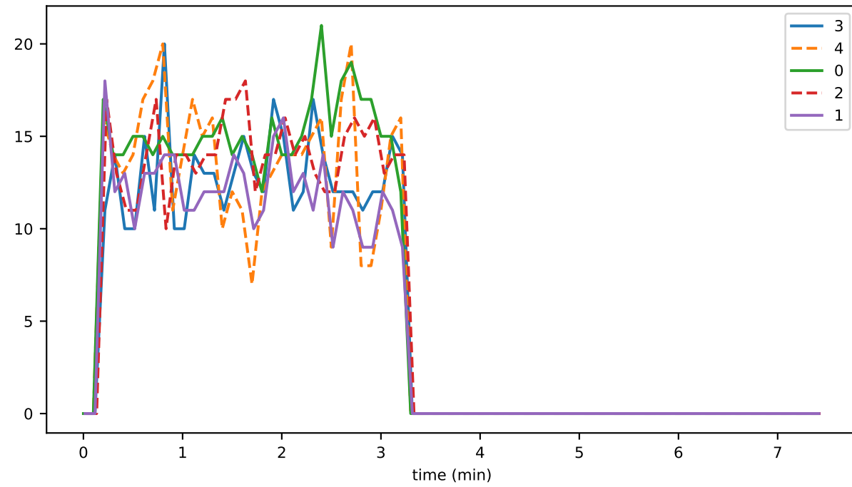
ev_per_syncRMAX
