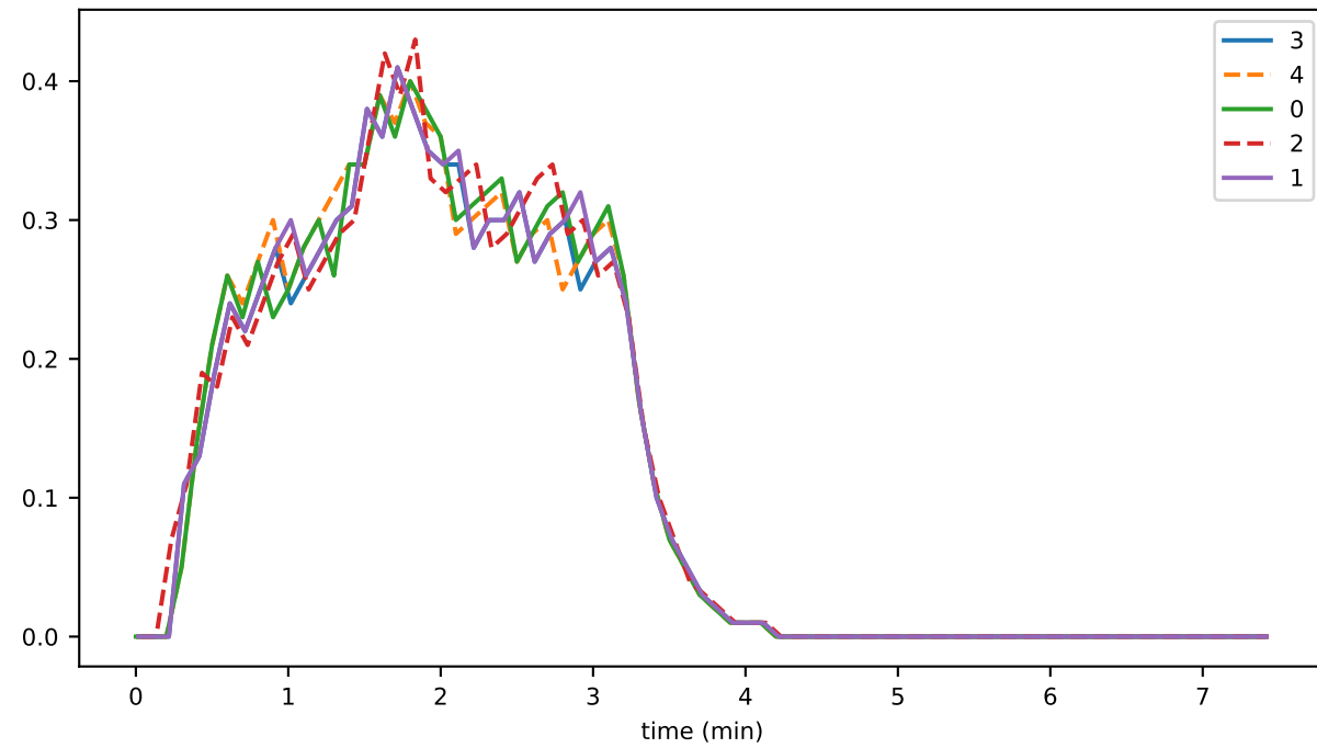
staleTransactions
