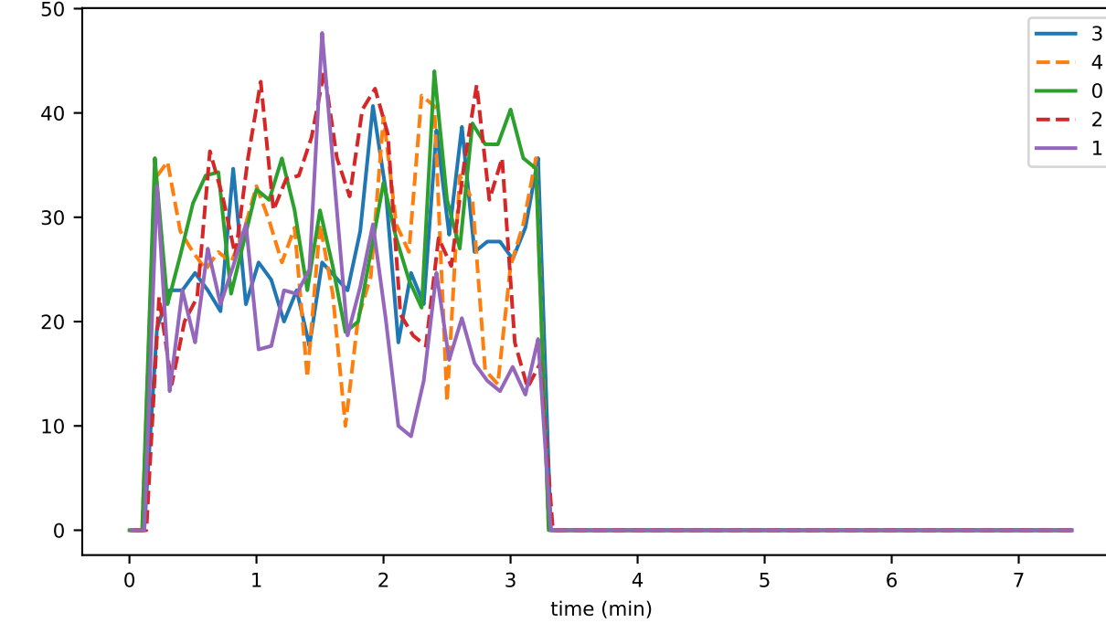
endsReconnectAsReceiver
