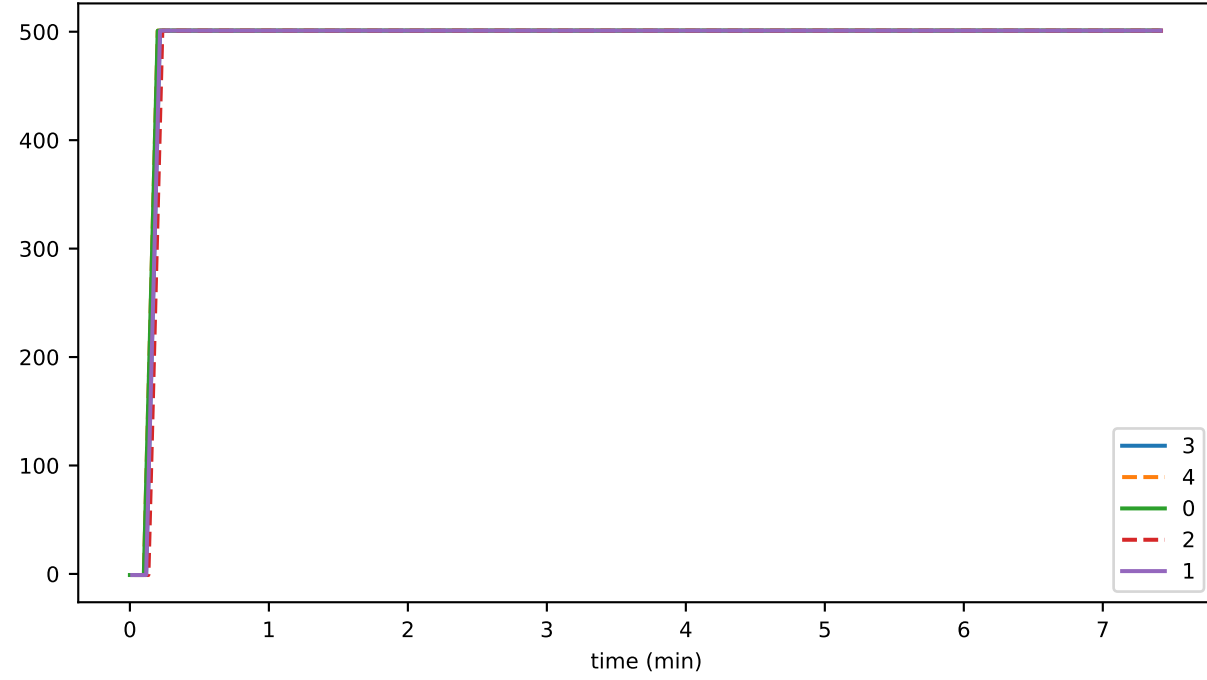
preconsensusEventFileYoungestIdentifier
