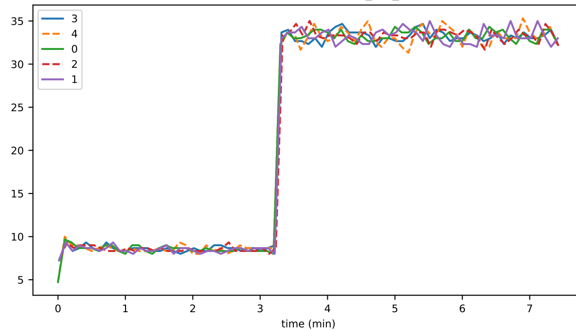
opportunitiesToInitiateSync_per_sec
