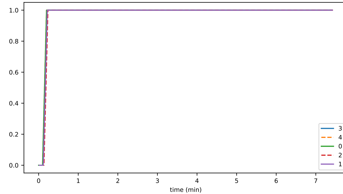
healthyNetworkFraction
