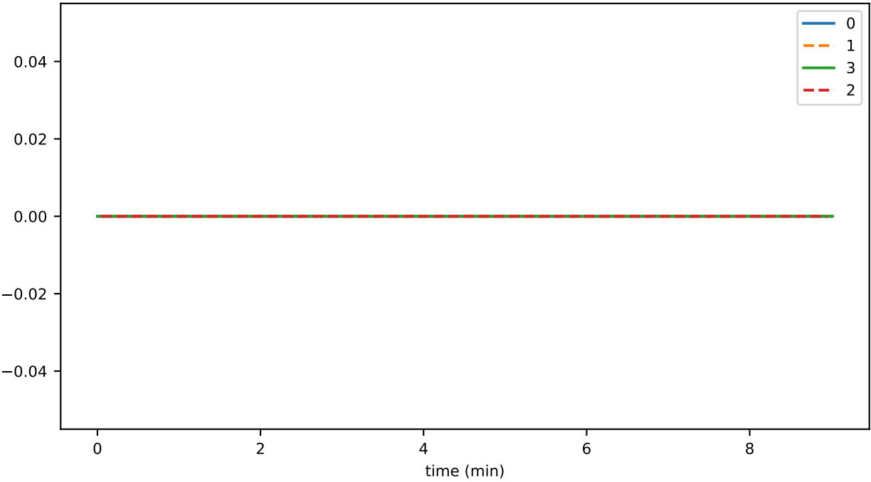
ds_compactions_level_5_hashesSavedSpaceMb_accounts
