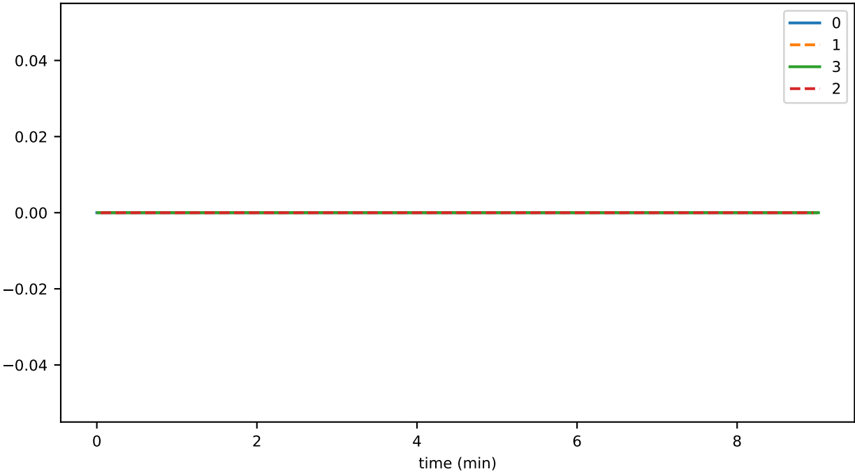
ds_compactions_level_5_hashesTimeMs_accounts
