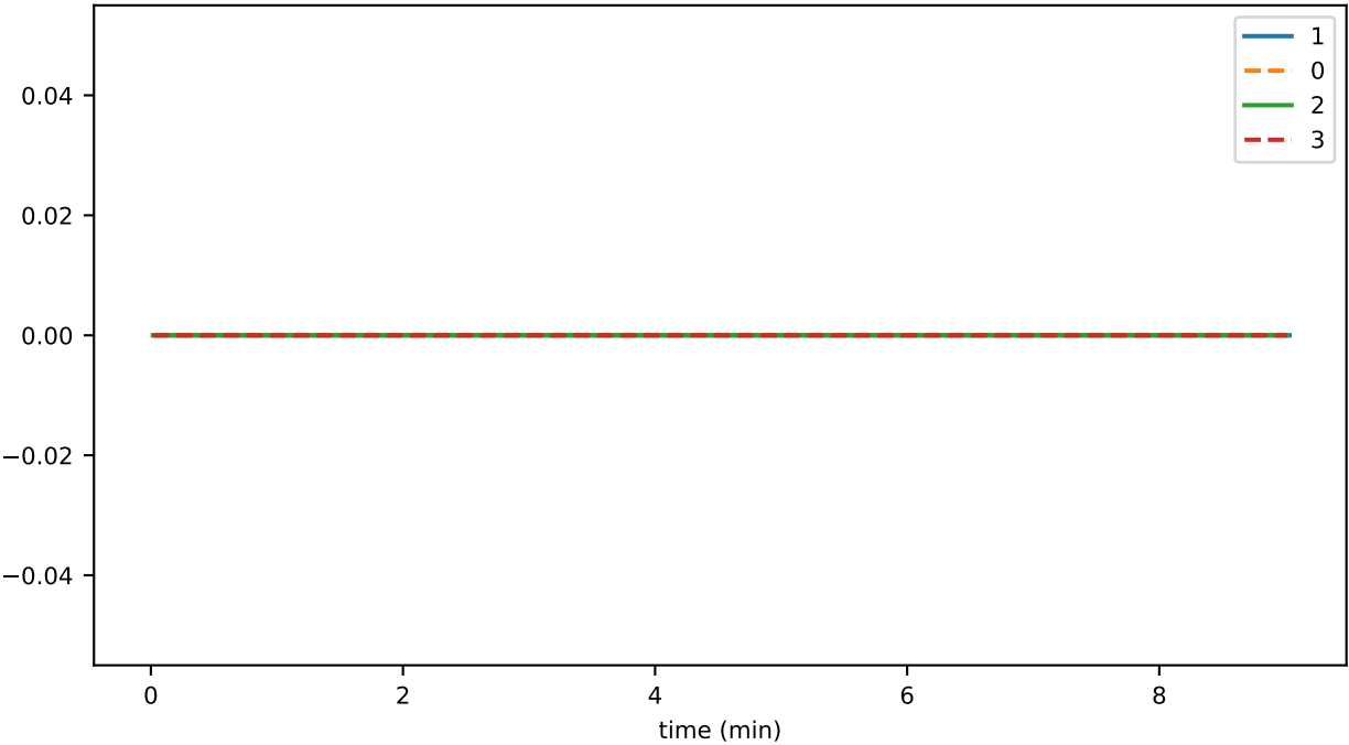
ds_files_level_1_hashesFileSizeByLevelMb_accounts
