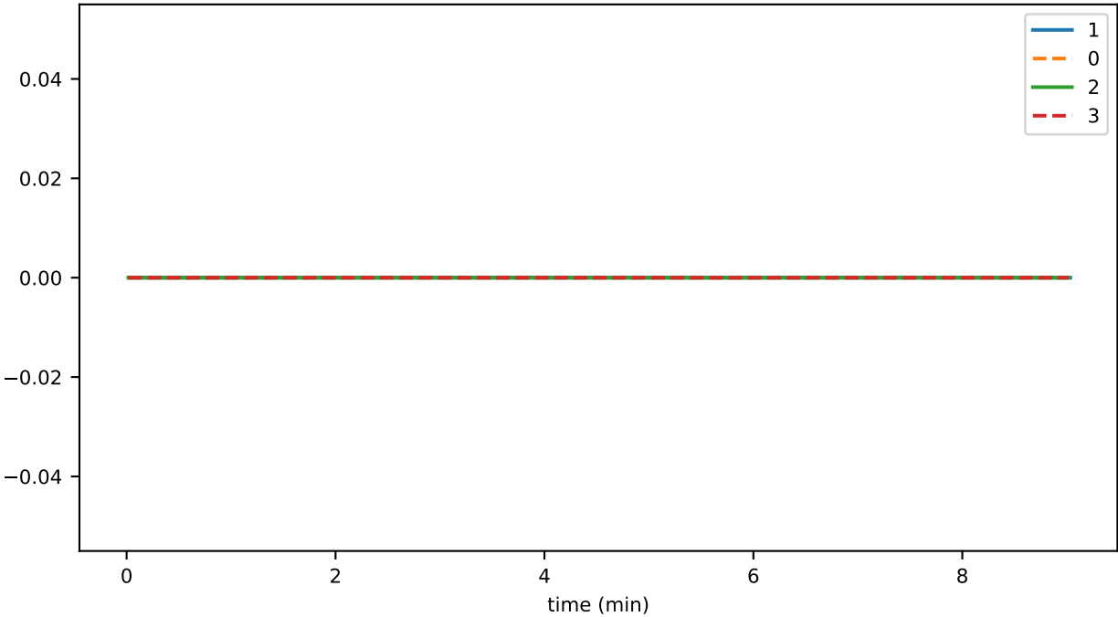
ds_files_level_1_leafKeysFileSizeByLevelMb_accounts
