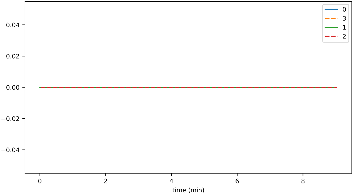
ds_files_level_5_leafKeysFileSizeByLevelMb_accounts
