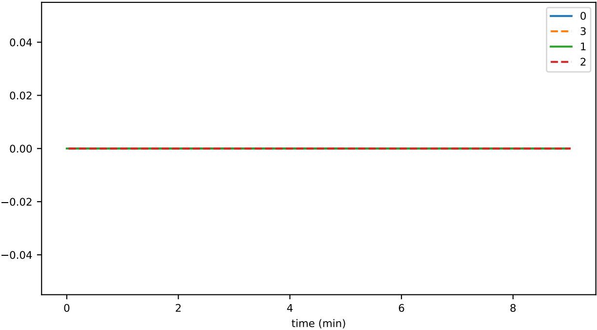
ds_files_level_5_hashesFileSizeByLevelMb_accounts
