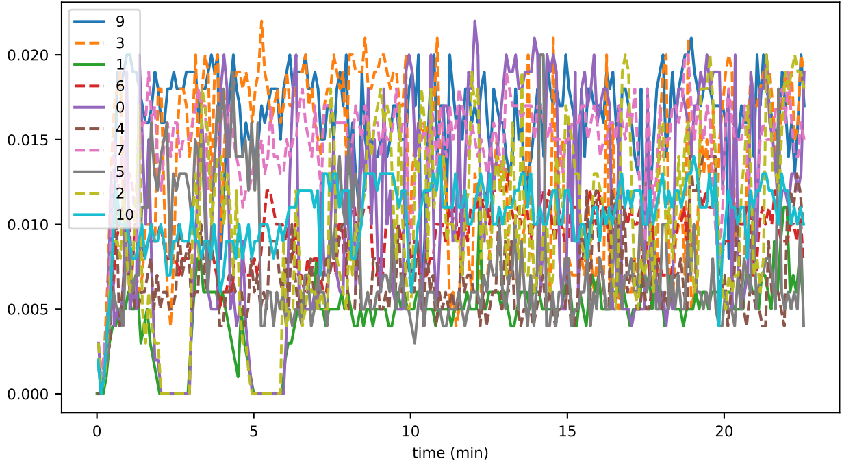
sync_phase_08_fraction_EXCHANGING_EVENTS
