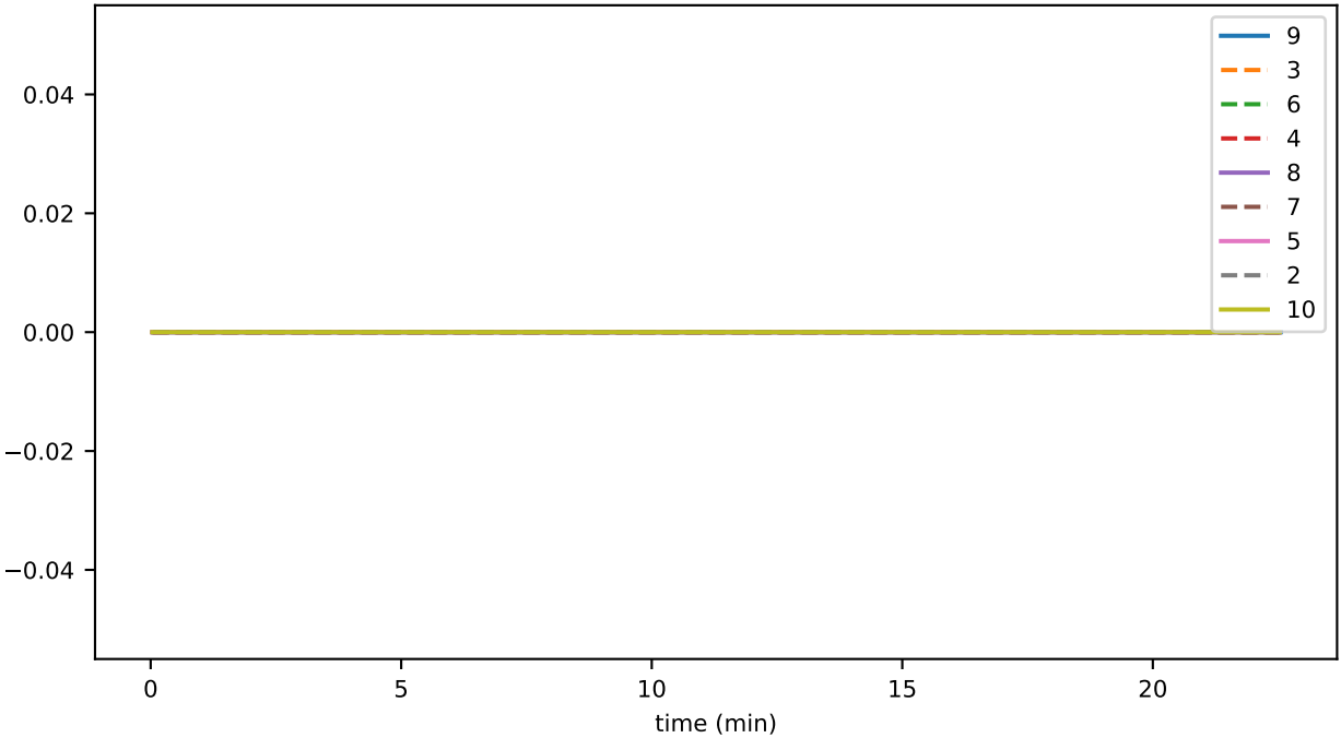
sync_phase_01_fraction_EXCHANGING_EVENTS
