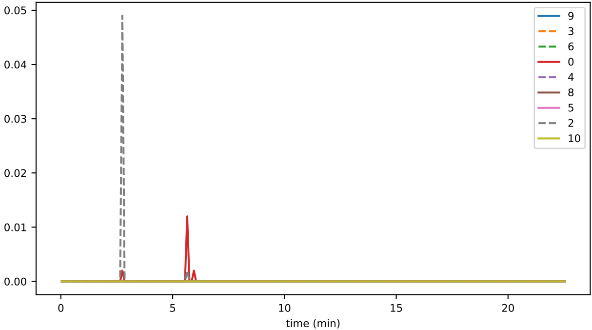
sync_phase_08_fraction_EXCHANGING_EVENTS
