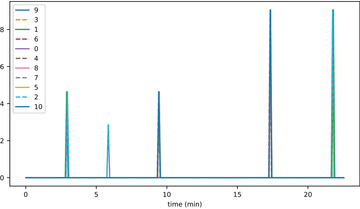
ds_flushes_leavesDeleted_accounts
