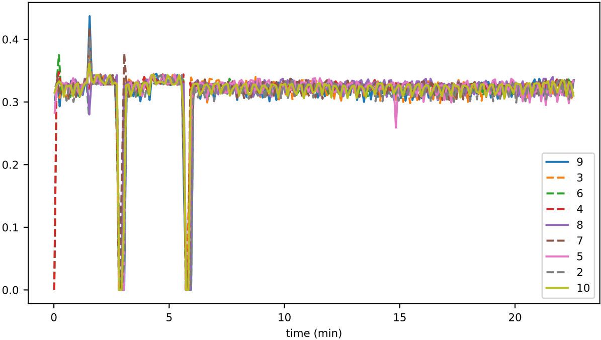
sync_phase_00_fraction_SENDING_EVENTS
