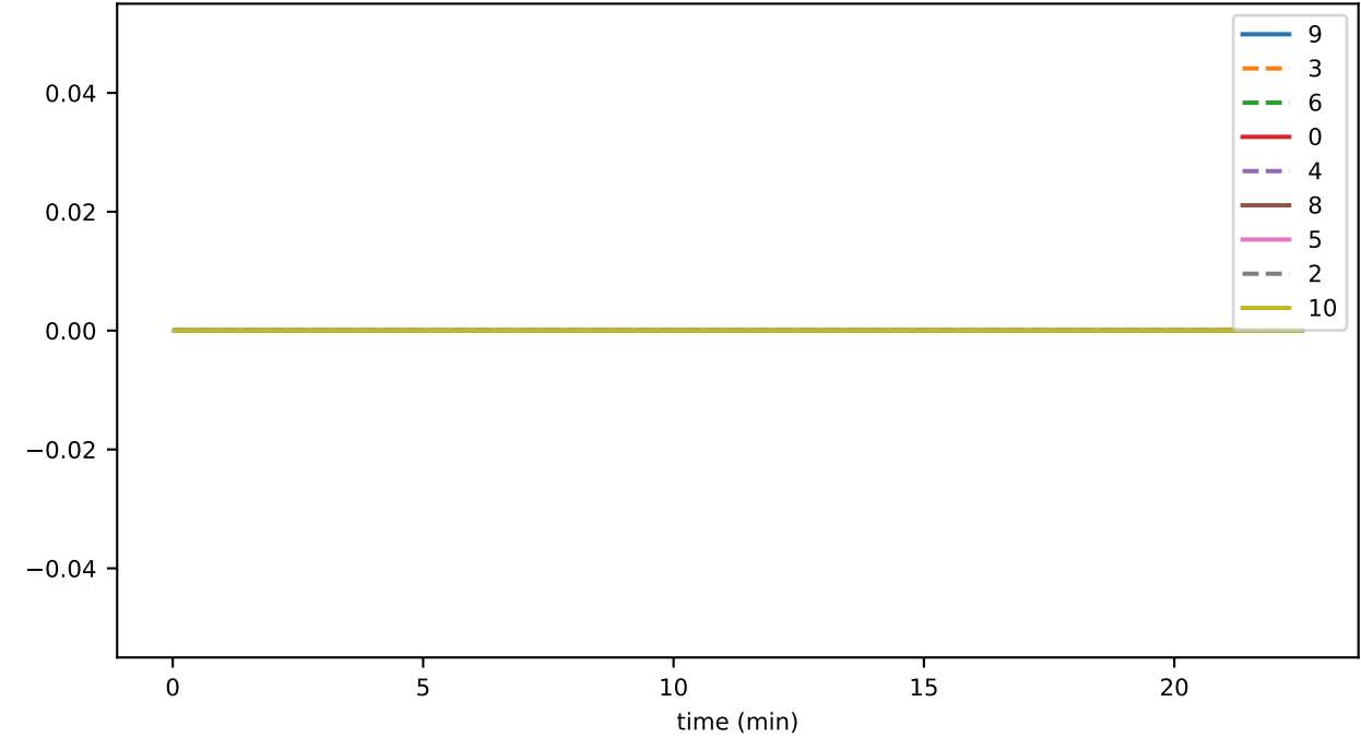
sync_phase_07_fraction_SENDING_EVENTS
