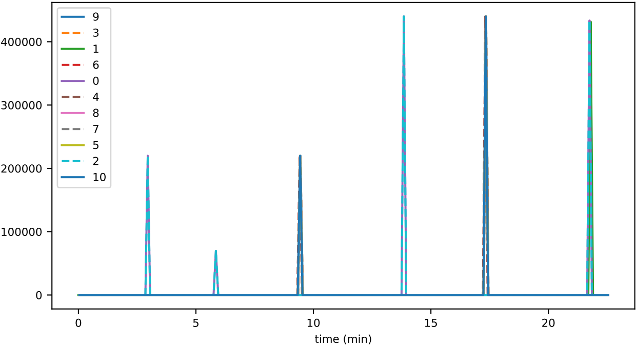
ds_flushes_leafKeysWritten_accounts
