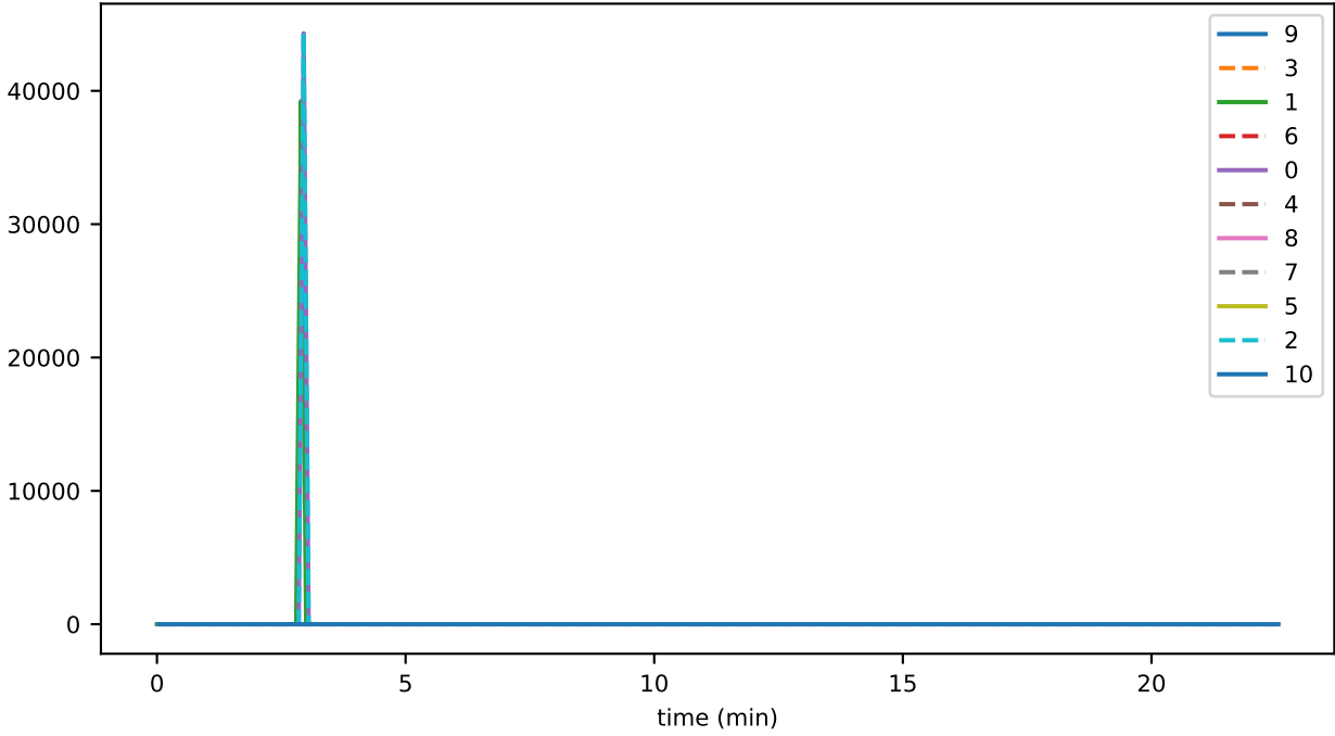
ds_flushes_leavesDeleted_accounts
