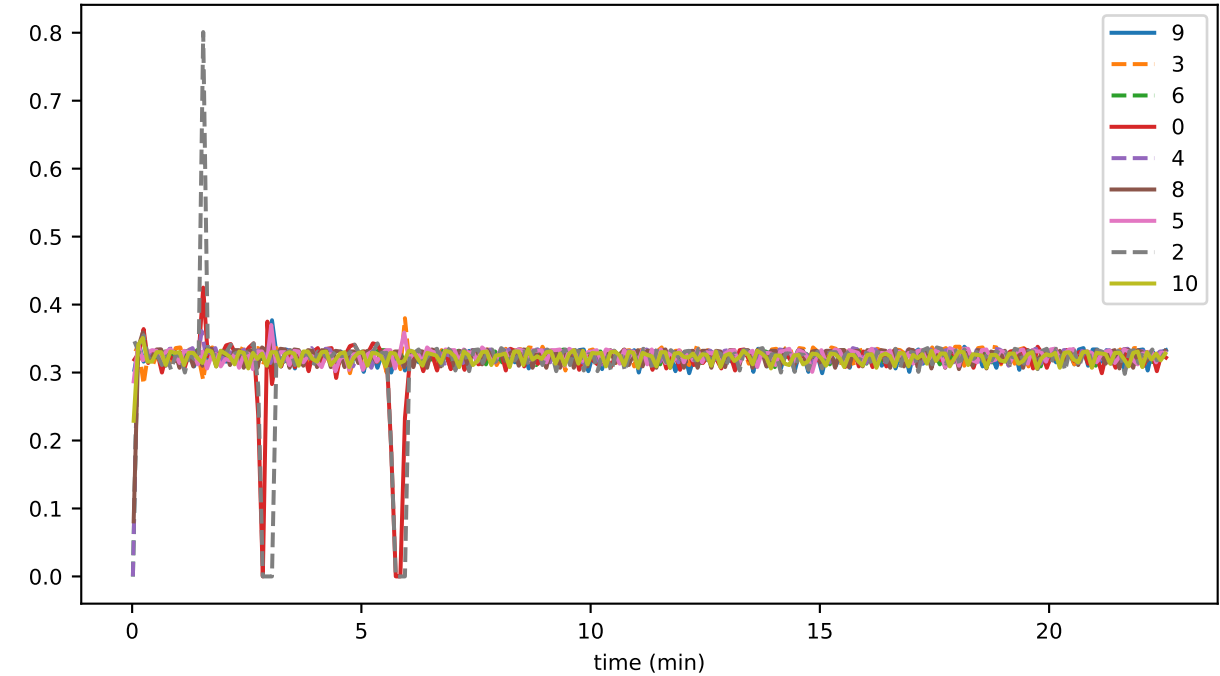
sync_phase_07_fraction_SENDING_EVENTS
