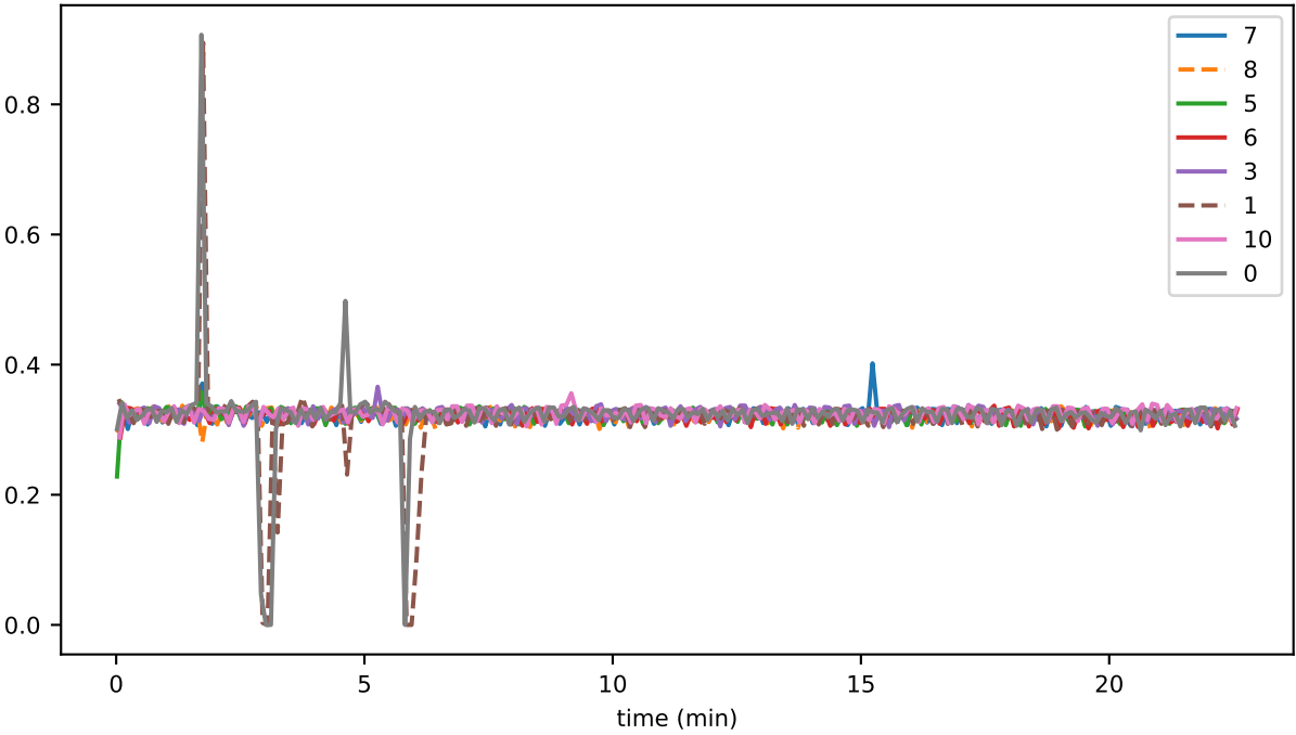
sync_phase_04_fraction_SENDING_EVENTS
