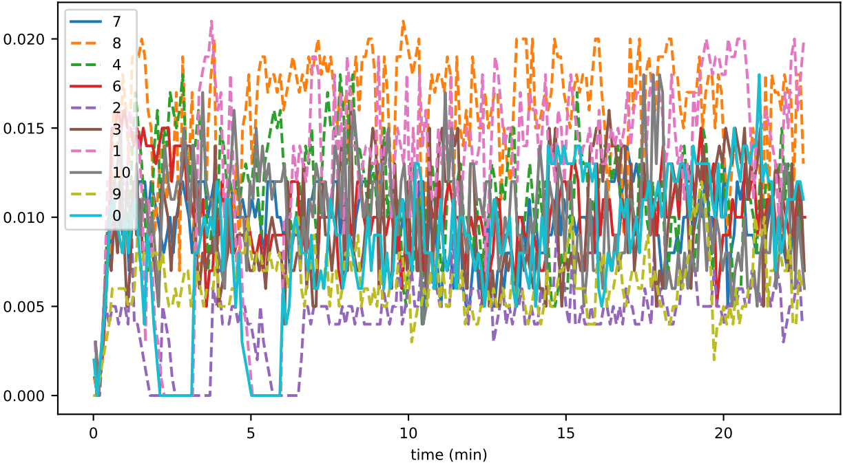
sync_phase_05_fraction_EXCHANGING_EVENTS
