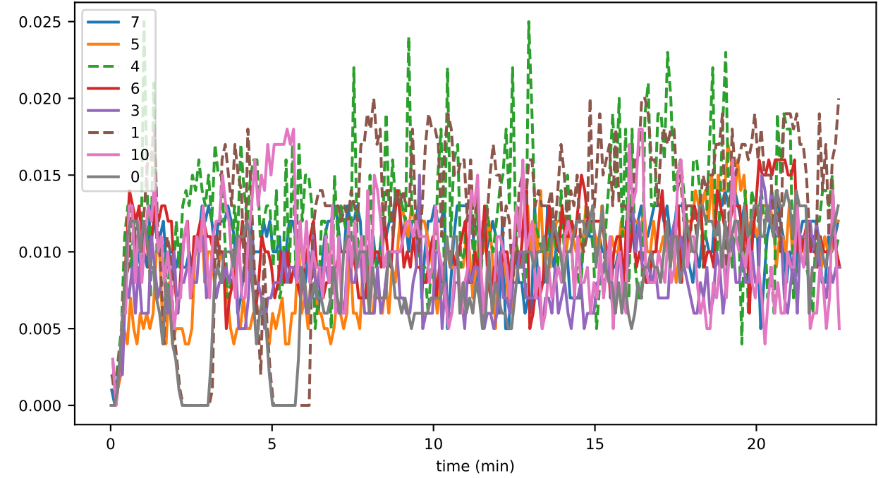
sync_phase_08_fraction_EXCHANGING_EVENTS
