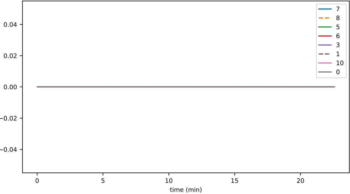
sync_phase_04_fraction_SENDING_EVENTS
