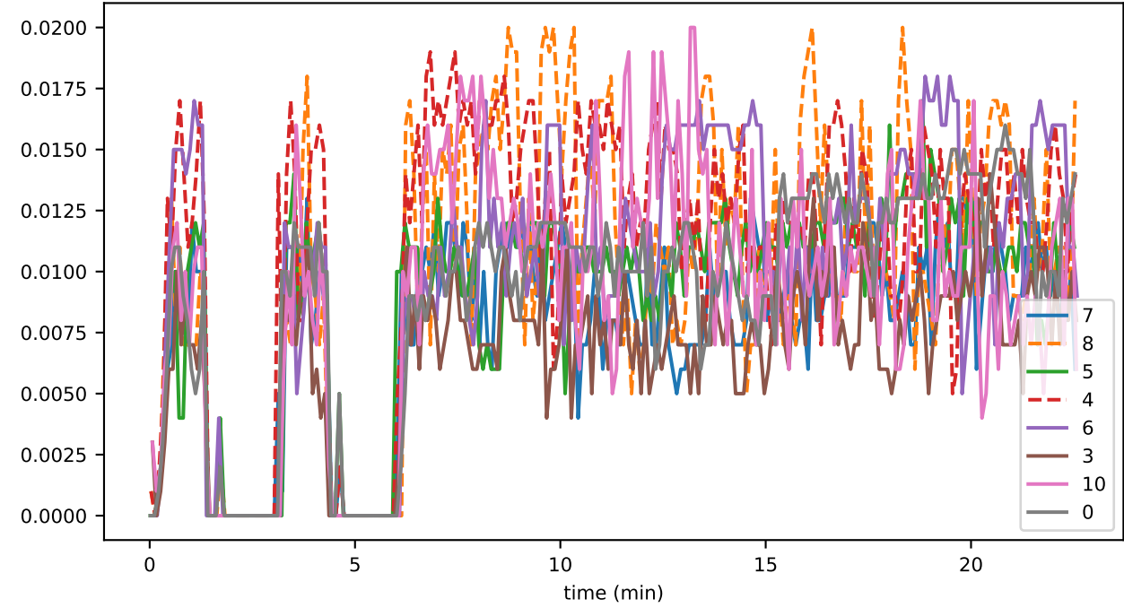
sync_phase_01_fraction_EXCHANGING_EVENTS
