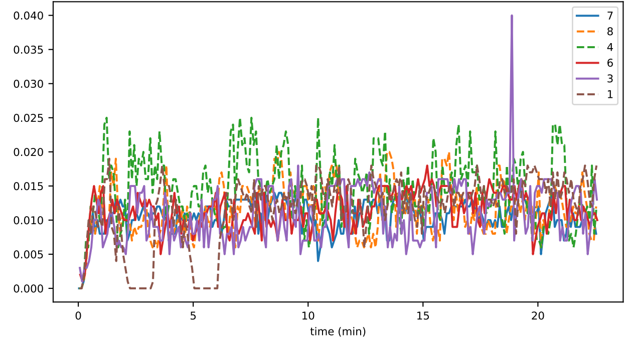
sync_phase_10_fraction_EXCHANGING_EVENTS
