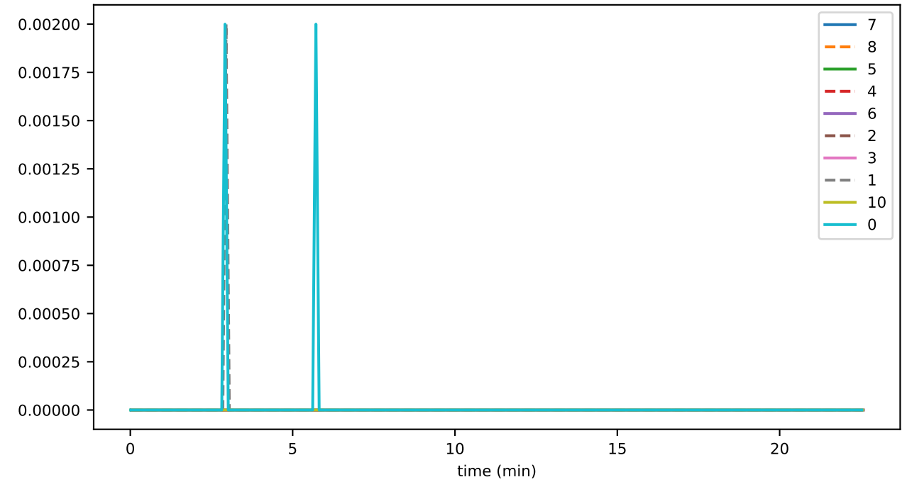
sync_phase_10_fraction_EXCHANGING_EVENTS
