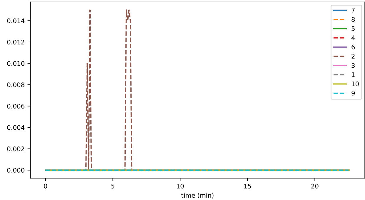
sync_phase_01_fraction_EXCHANGING_EVENTS
