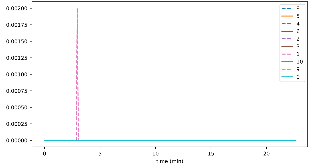
sync_phase_08_fraction_EXCHANGING_EVENTS
