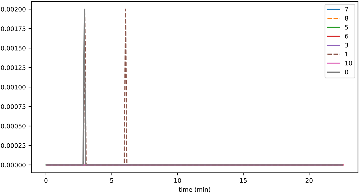
sync_phase_05_fraction_EXCHANGING_EVENTS
