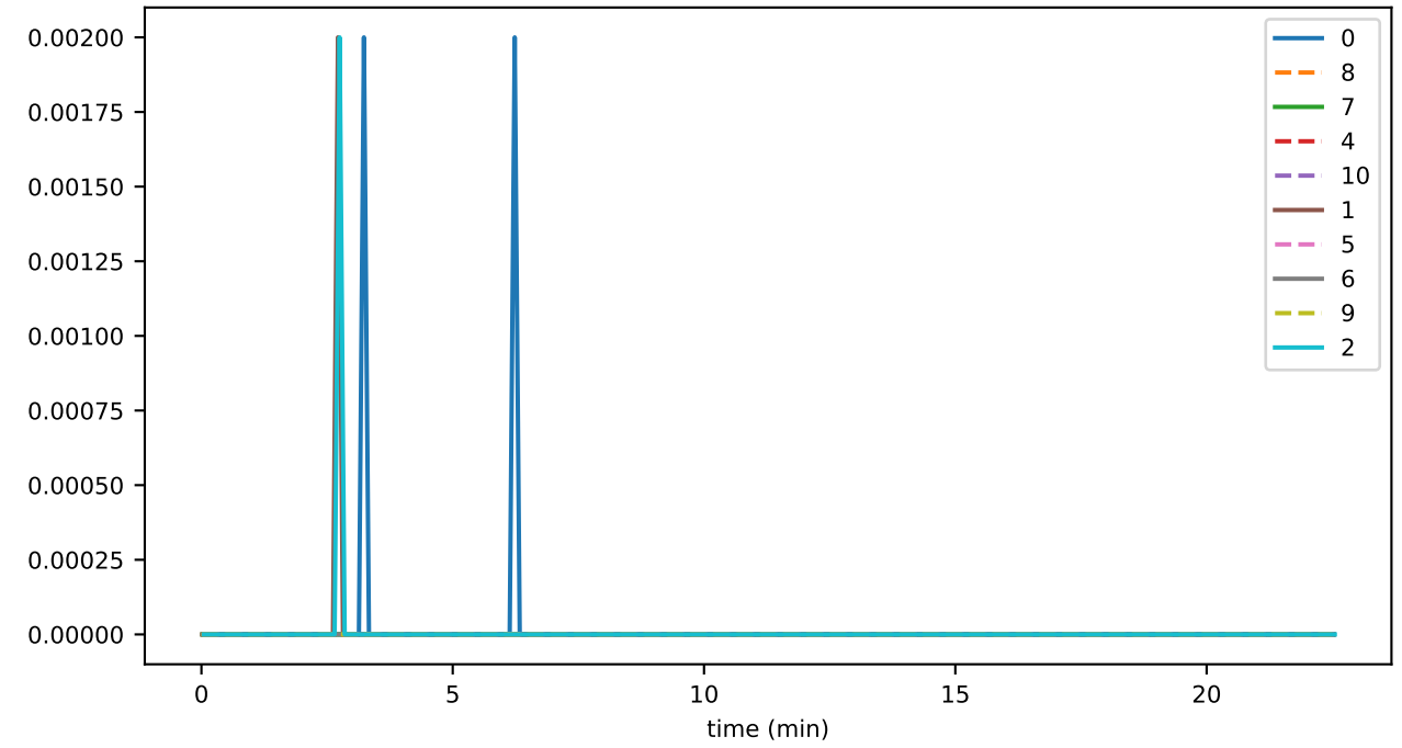
sync_phase_04_fraction_EXCHANGING_EVENTS
