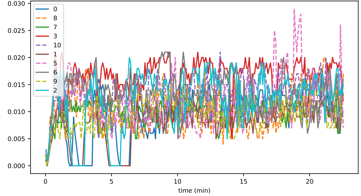
sync_phase_04_fraction_EXCHANGING_EVENTS
