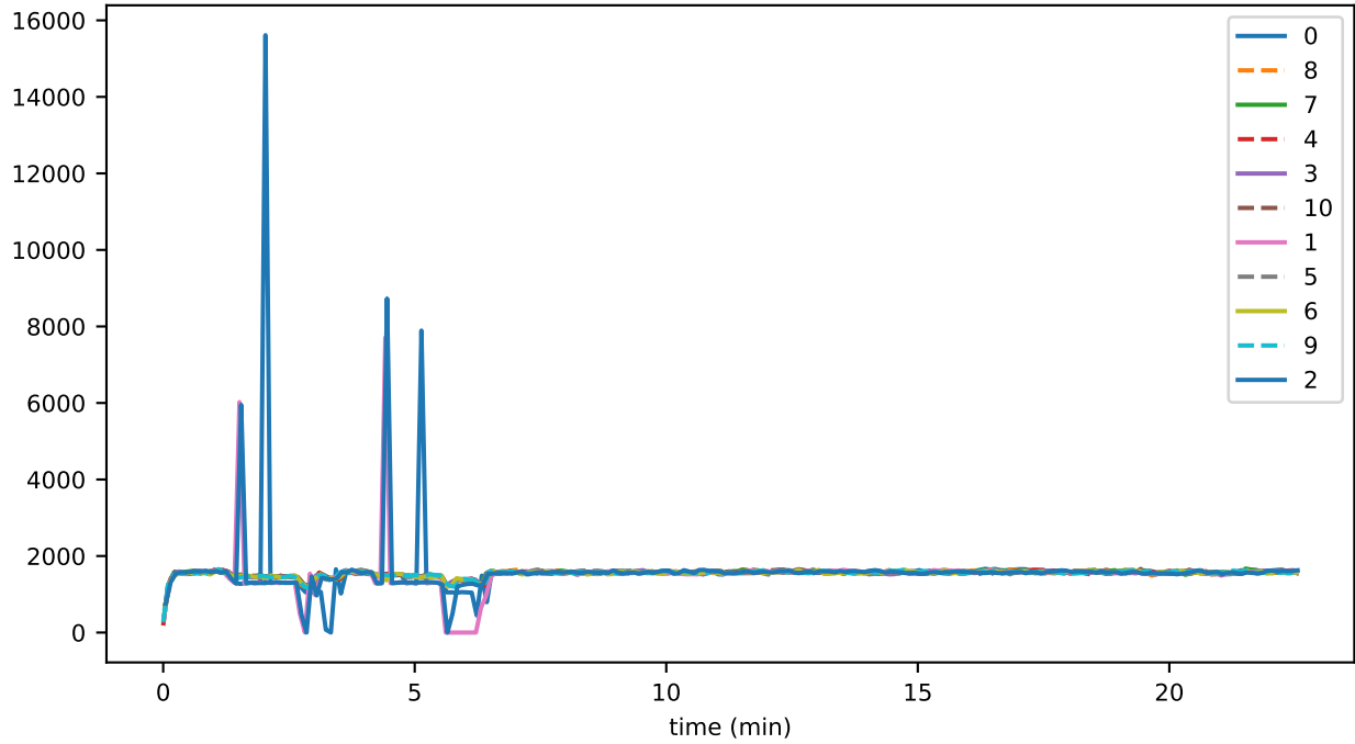
ds_compactions_level_0_hashesTimeMs_accounts
