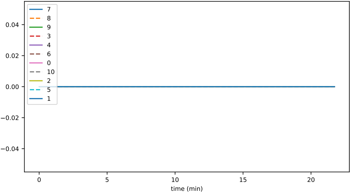
ds_files_totalSizeMb_accounts
