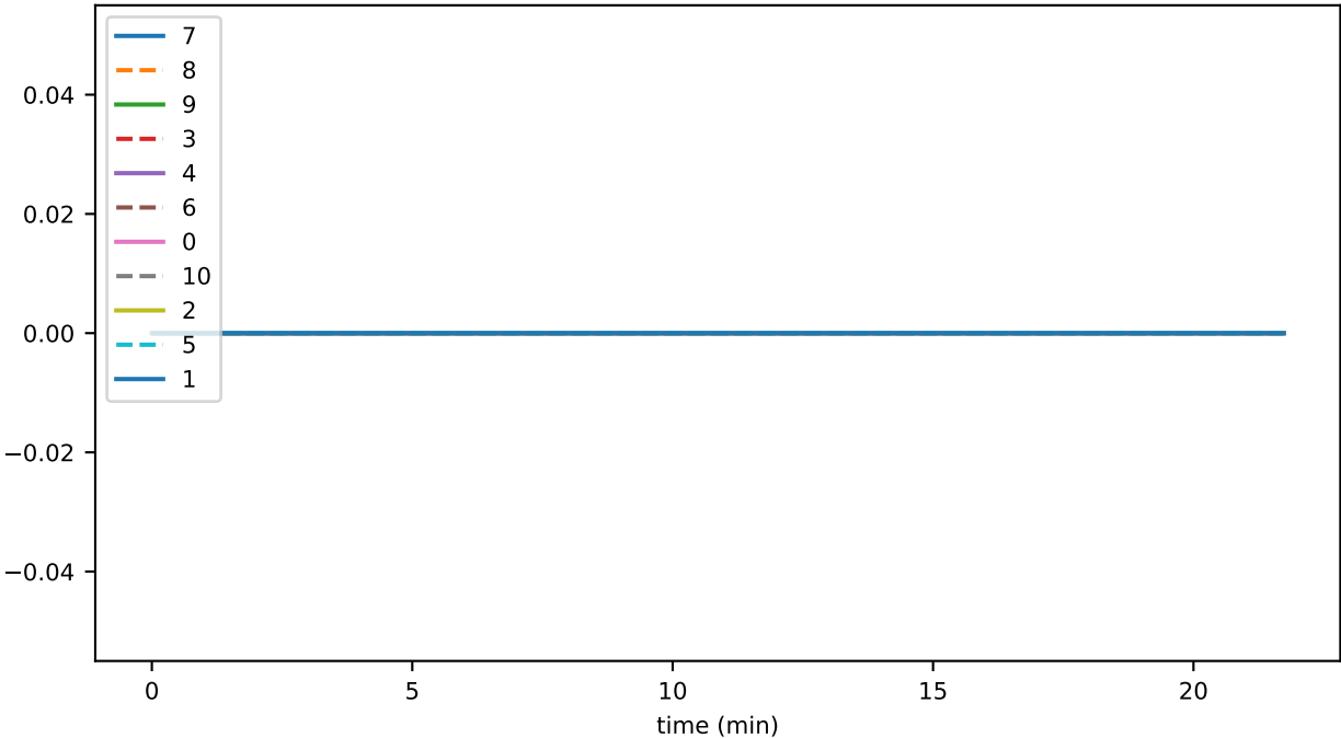
ds_flushes_hashesStoreFileSizeMb_accounts
