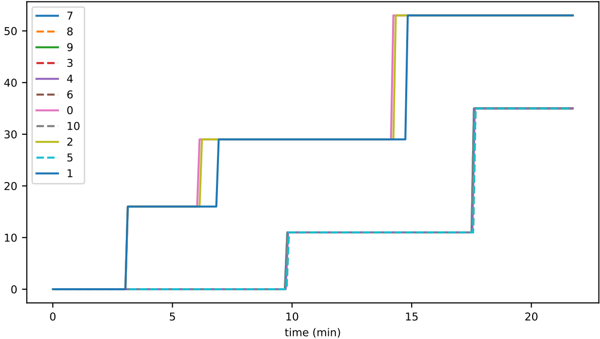
ds_files_totalSizeMb_accounts
