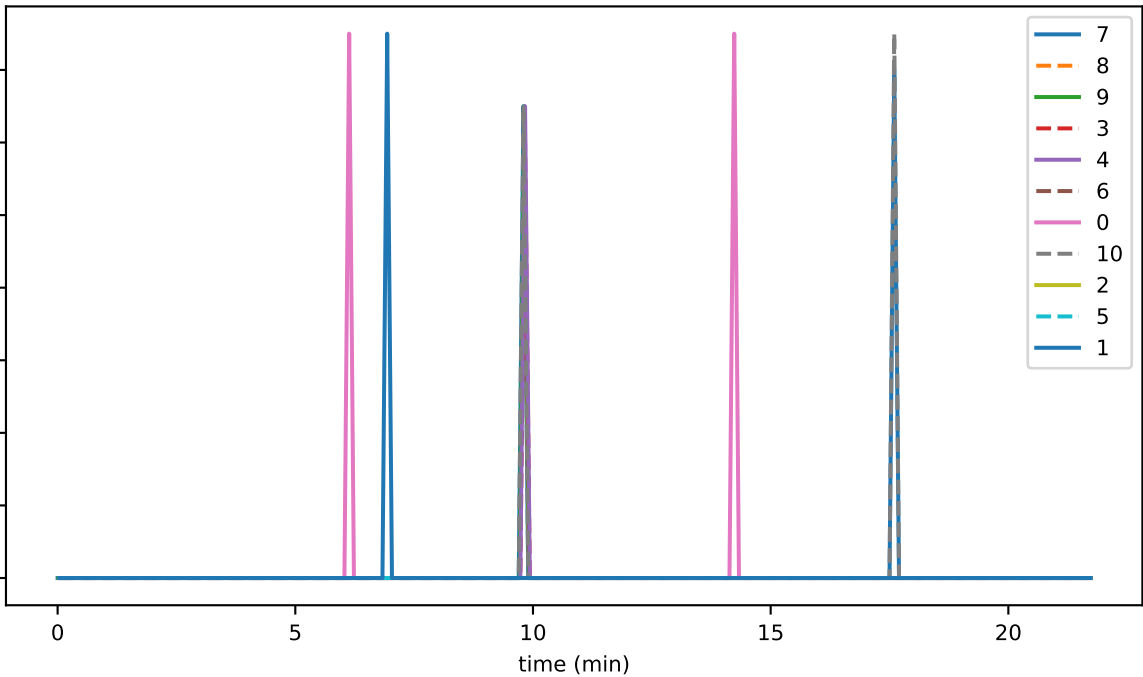
ds_flushes_hashesStoreFileSizeMb_accounts
