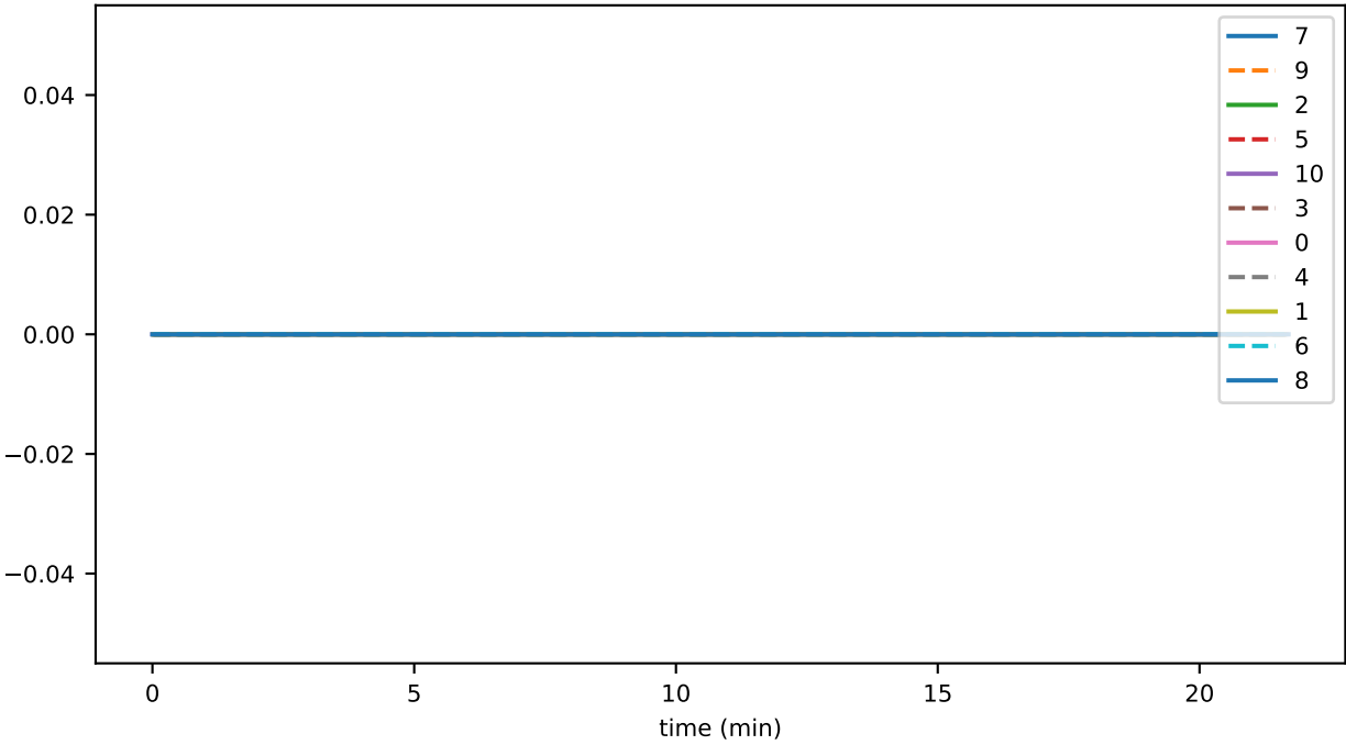
ds_flushes_hashesStoreFileSizeMb_accounts
