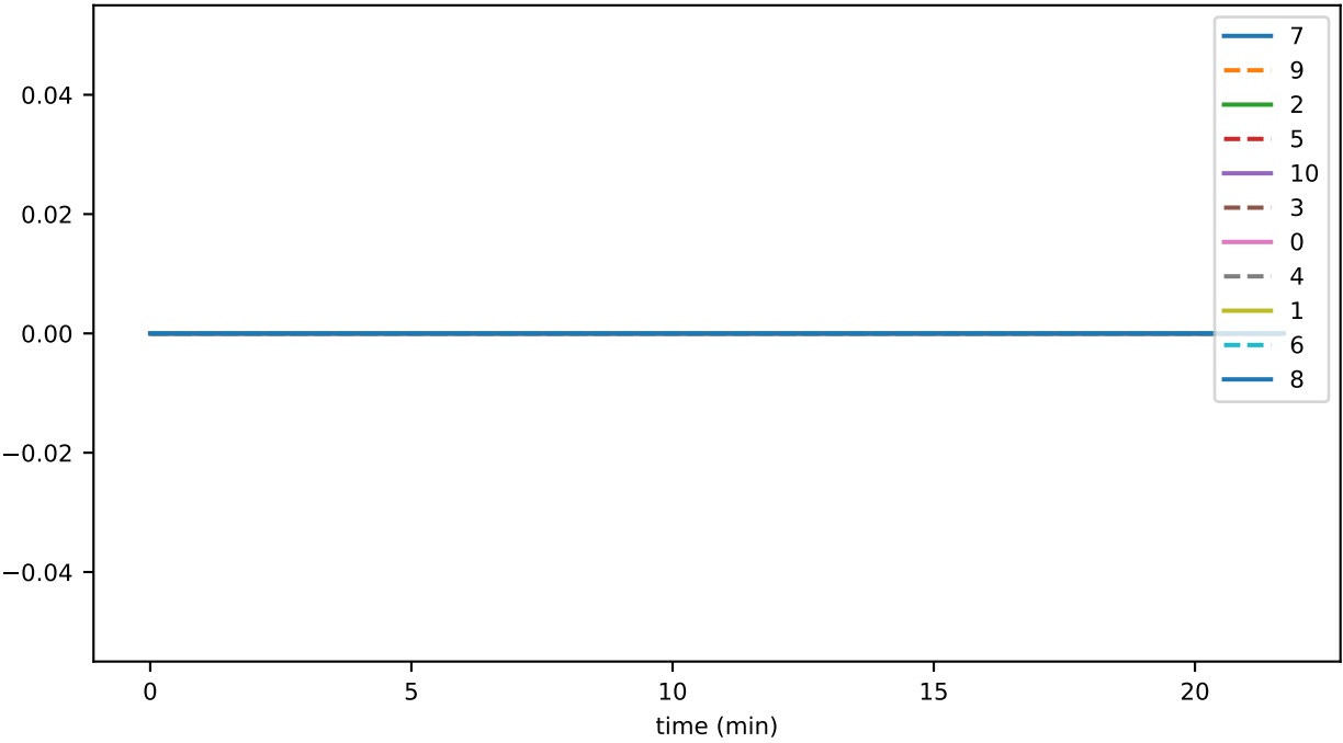
ds_files_totalSizeMb_accounts
