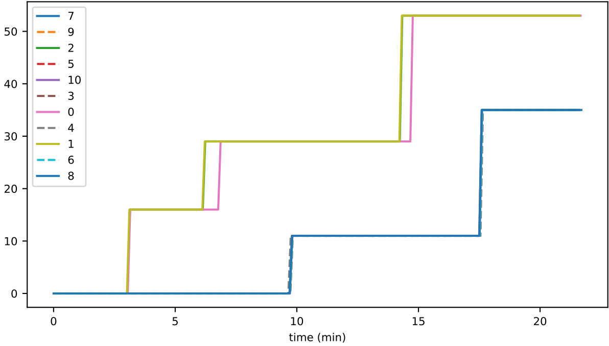
ds_files_totalSizeMb_accounts
