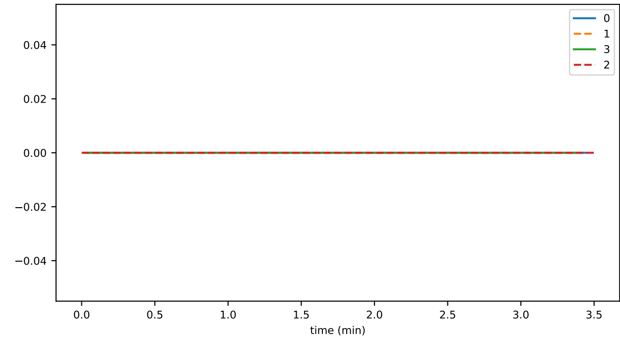
preconsensusEventAverageFileSpan
