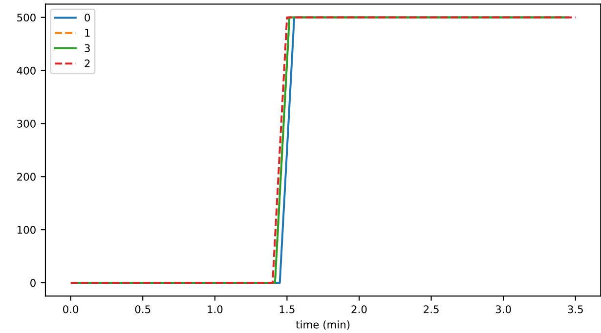
preconsensusEventAverageFileSpan
