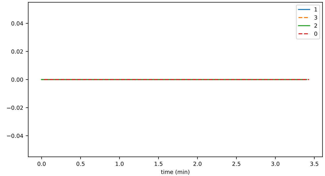
preconsensusEventAverageFileSpan
