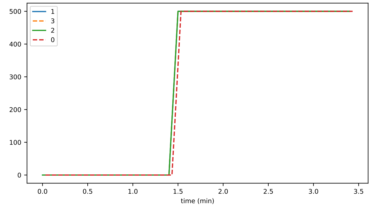
preconsensusEventAverageFileSpan
