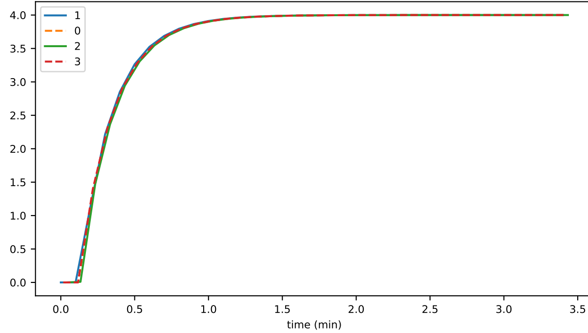
tips_per_sync
