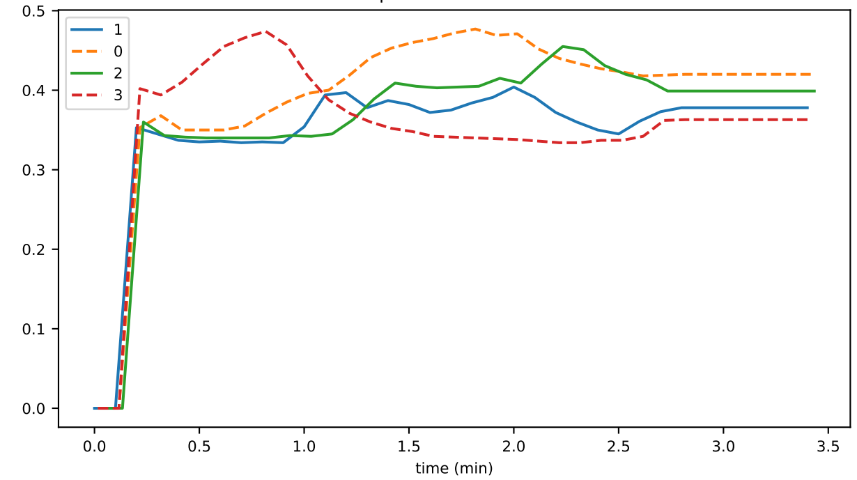
tipsetAdvancement
