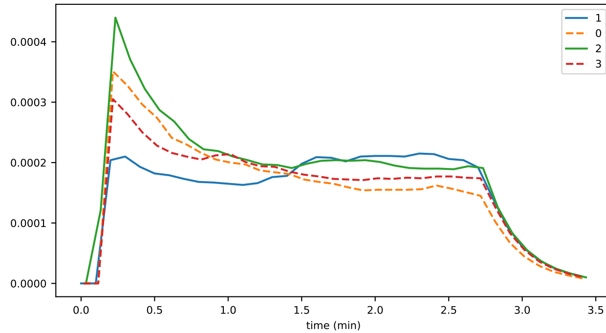
tips_per_sync
