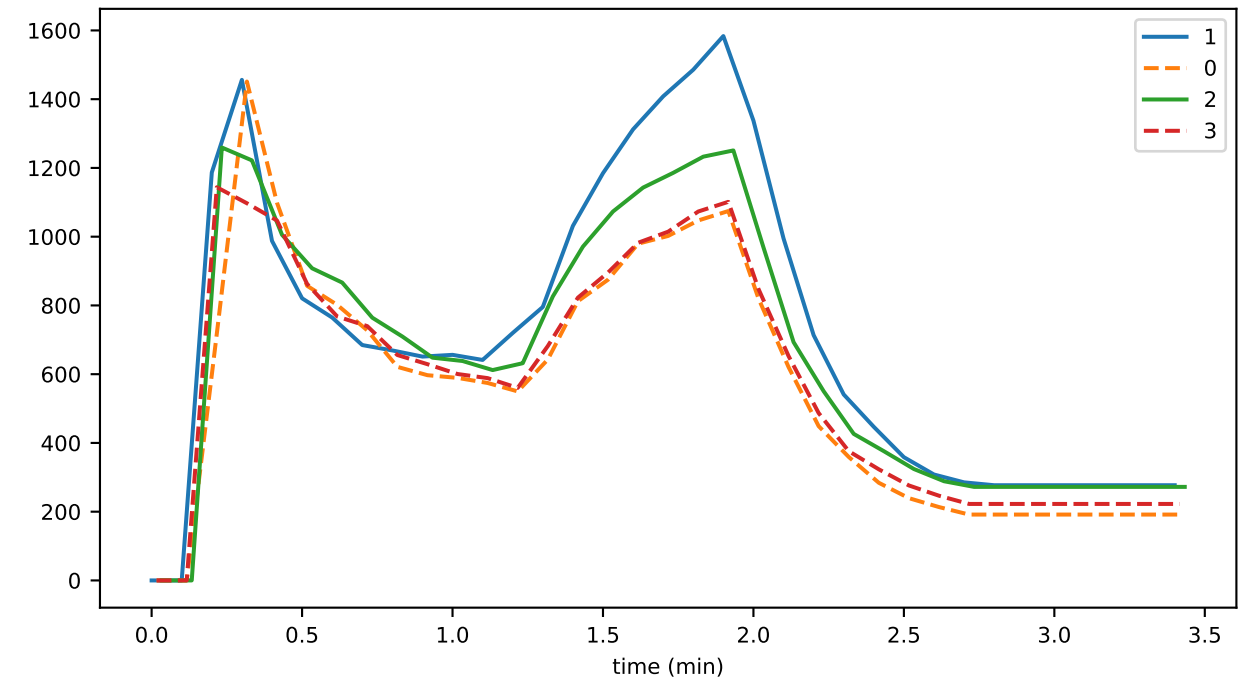
tipsetAdvancement
