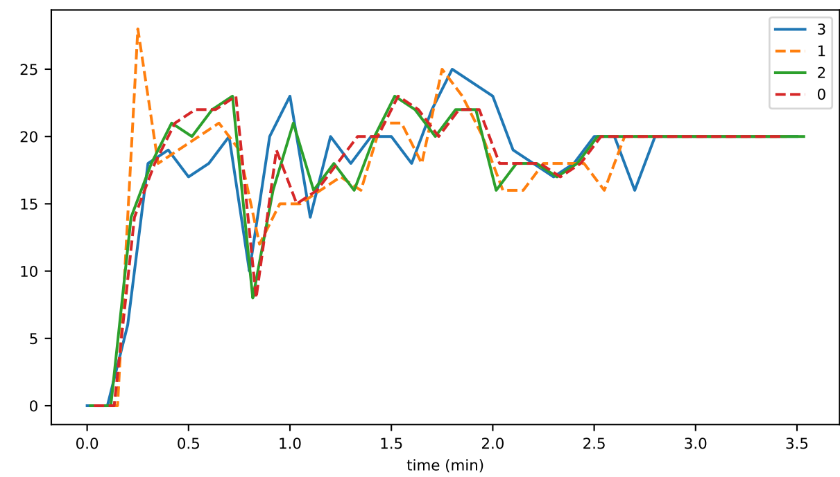
eventsPerRound
