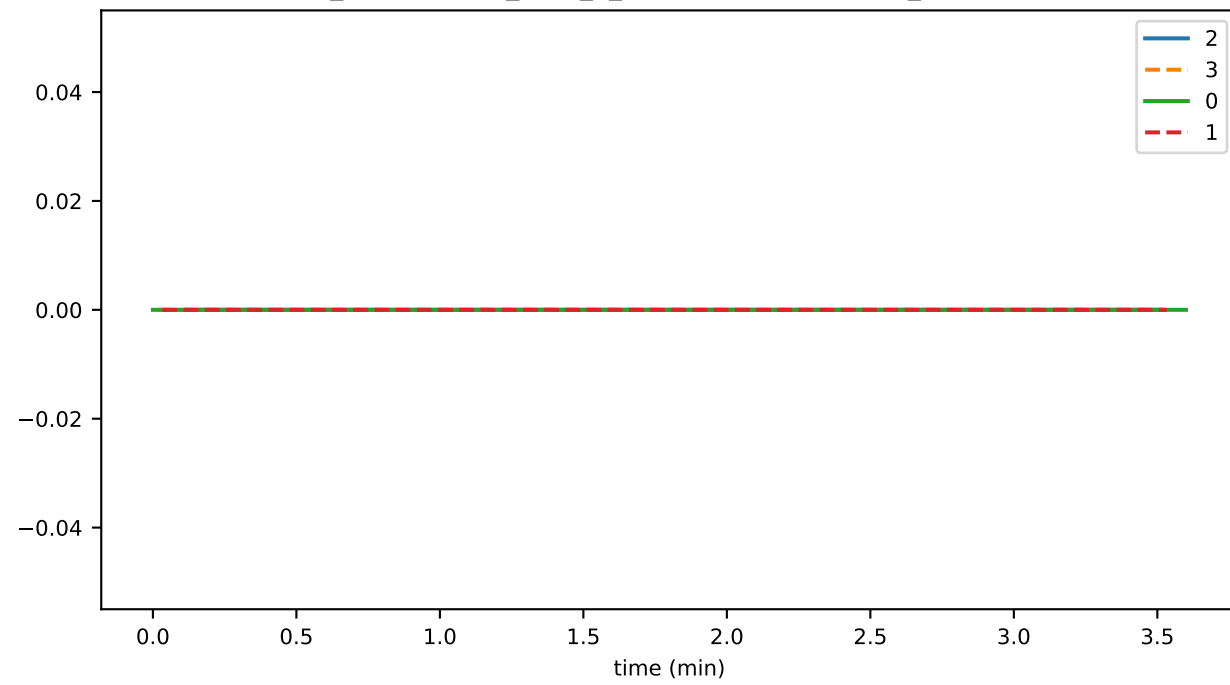
ds_compactions_level_0_hashesSavedSpaceMb_accounts
