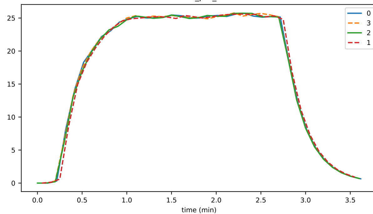
events_per_sec
