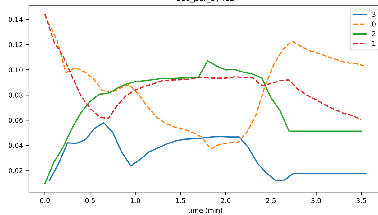
sec_per_sync1
