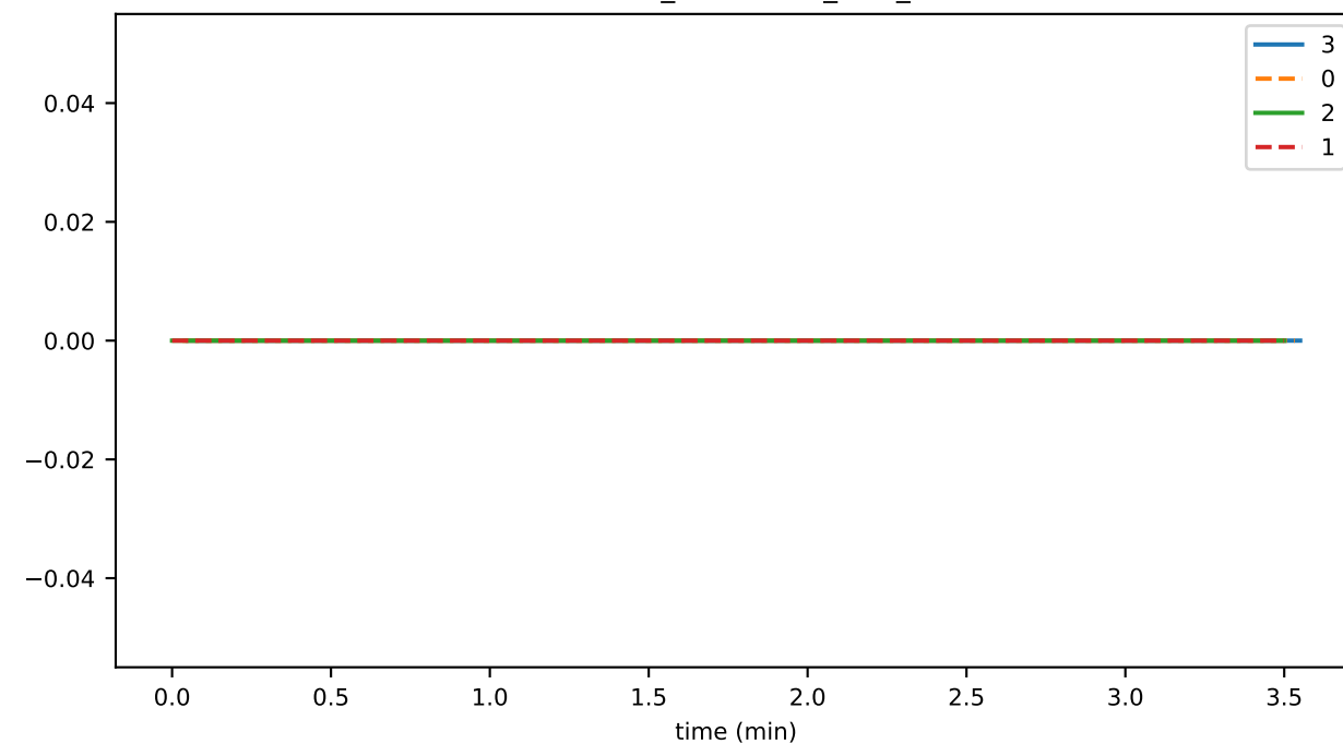
events_per_sec
