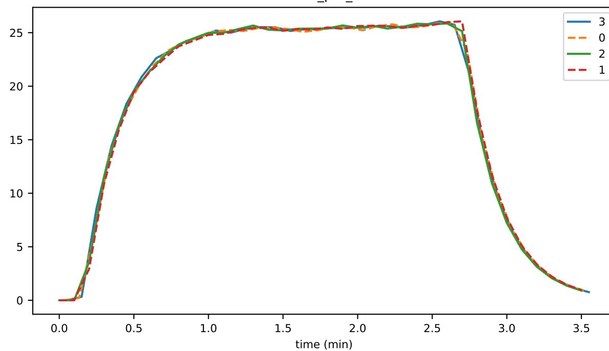
events_per_sec
