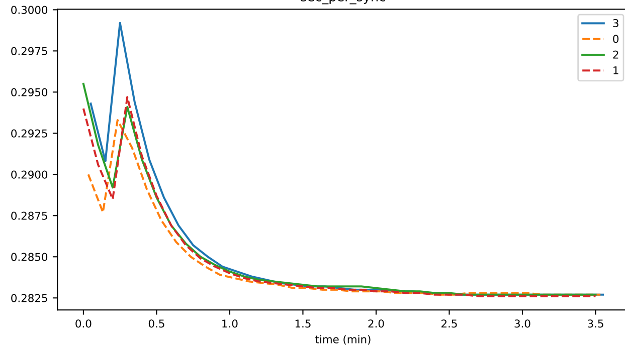
sec_per_sync
