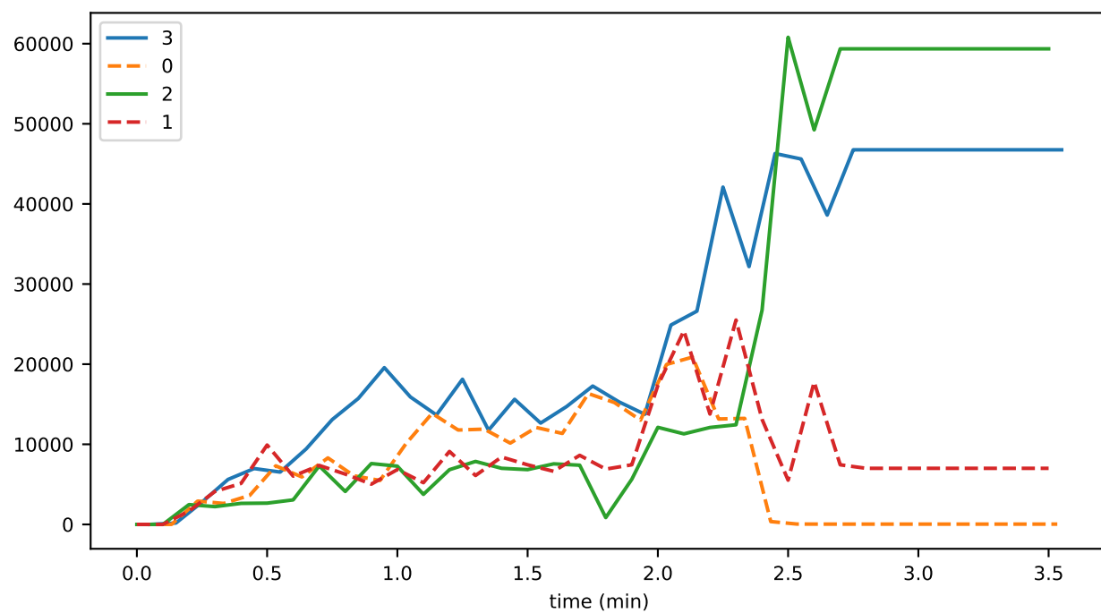
eventRecRate
