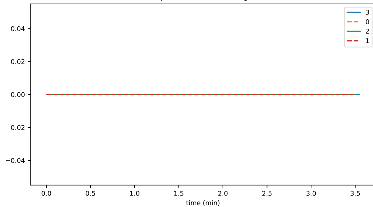
sec_per_sync
