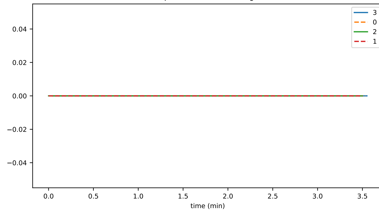
sec_per_sync1
