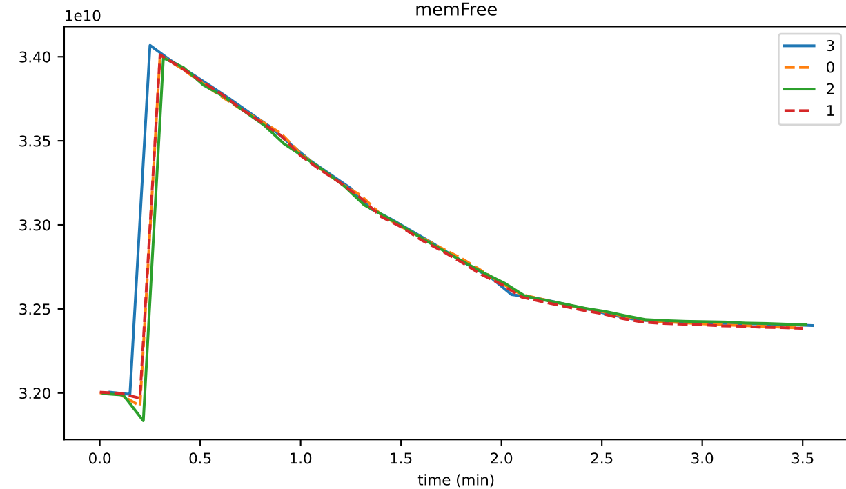
memFree
