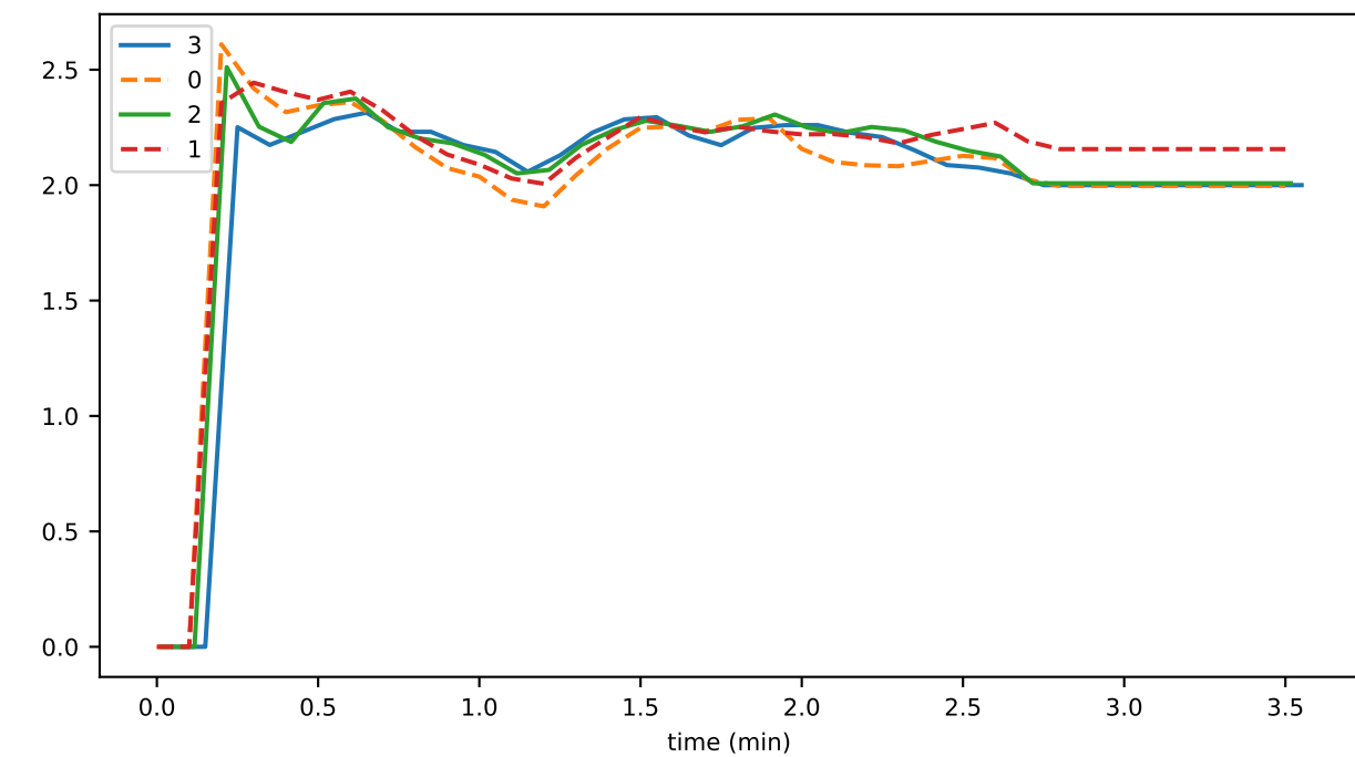
memFree
