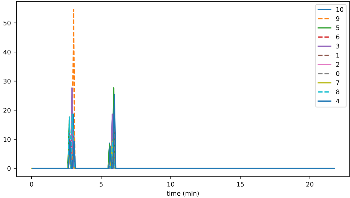
ds_compactions_level_0_hashesSavedSpaceMb_accounts
