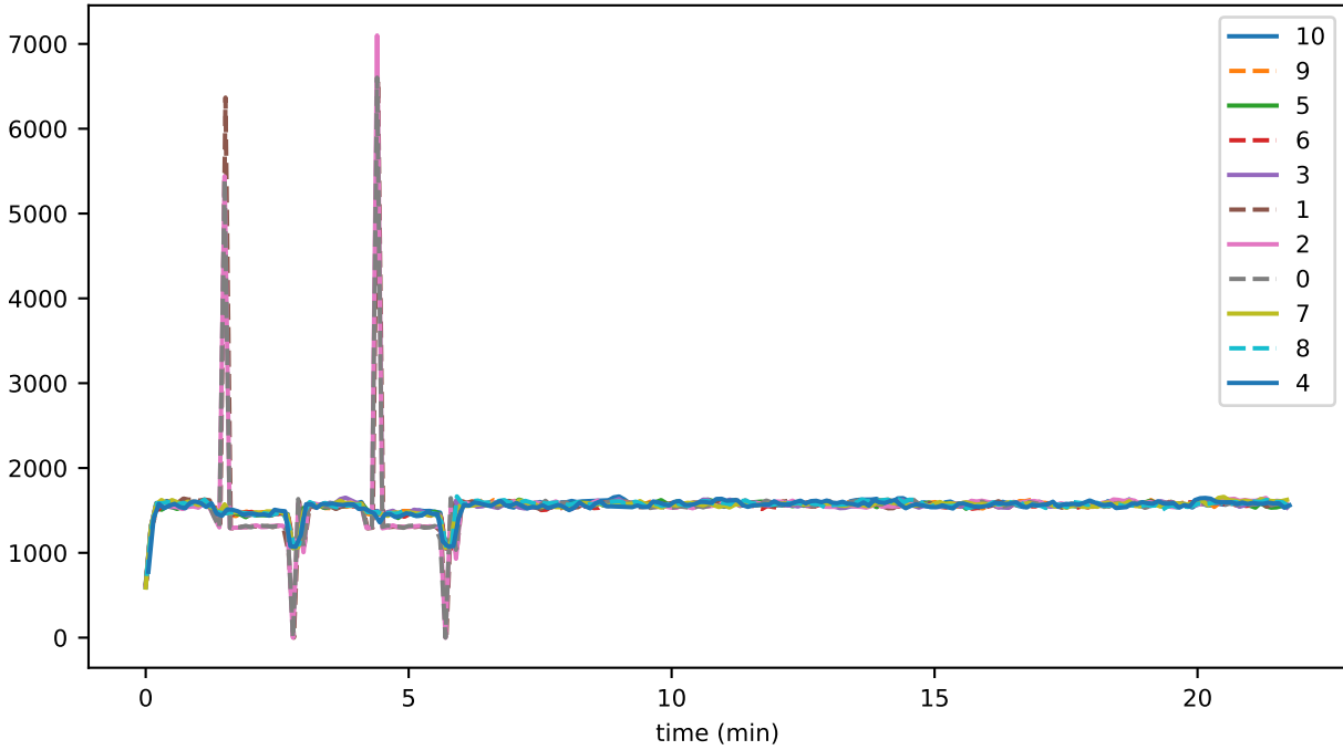
ds_compactions_level_0_hashesTimeMs_accounts
