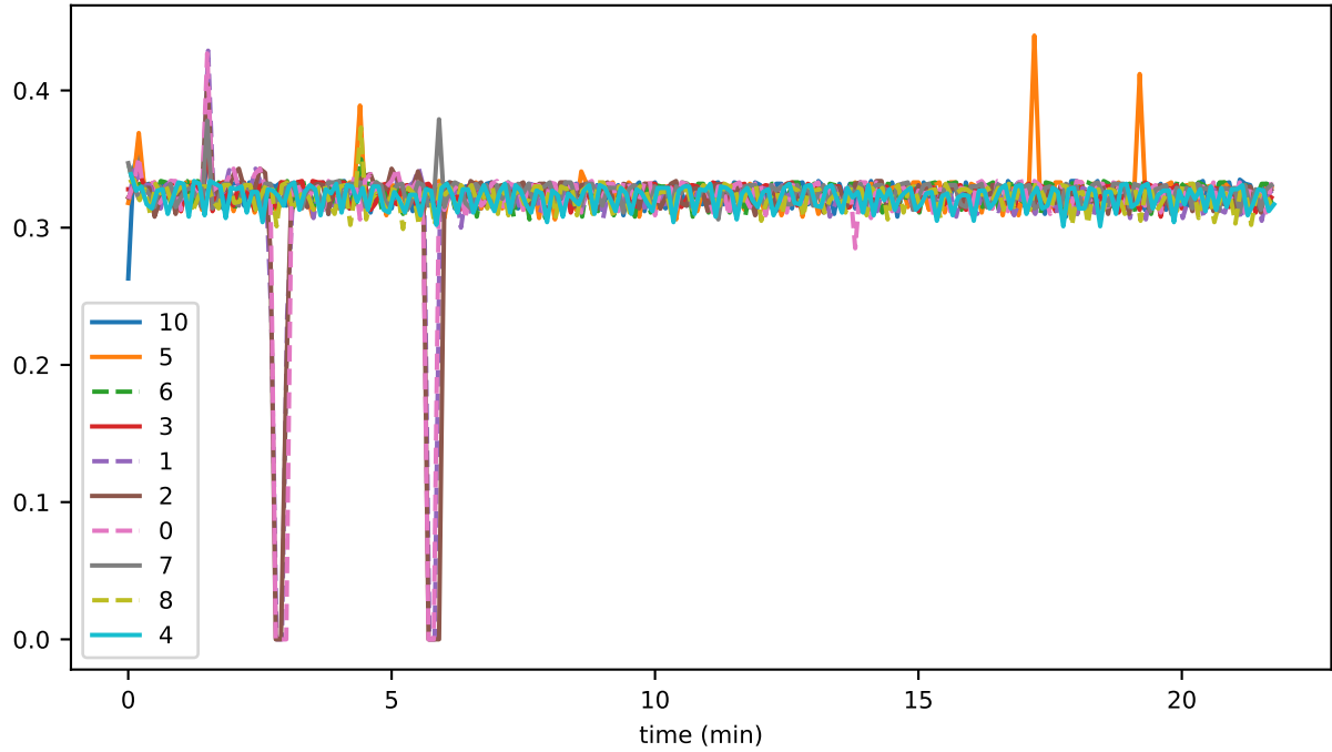
sync_phase_09_fraction_SENDING_EVENTS
