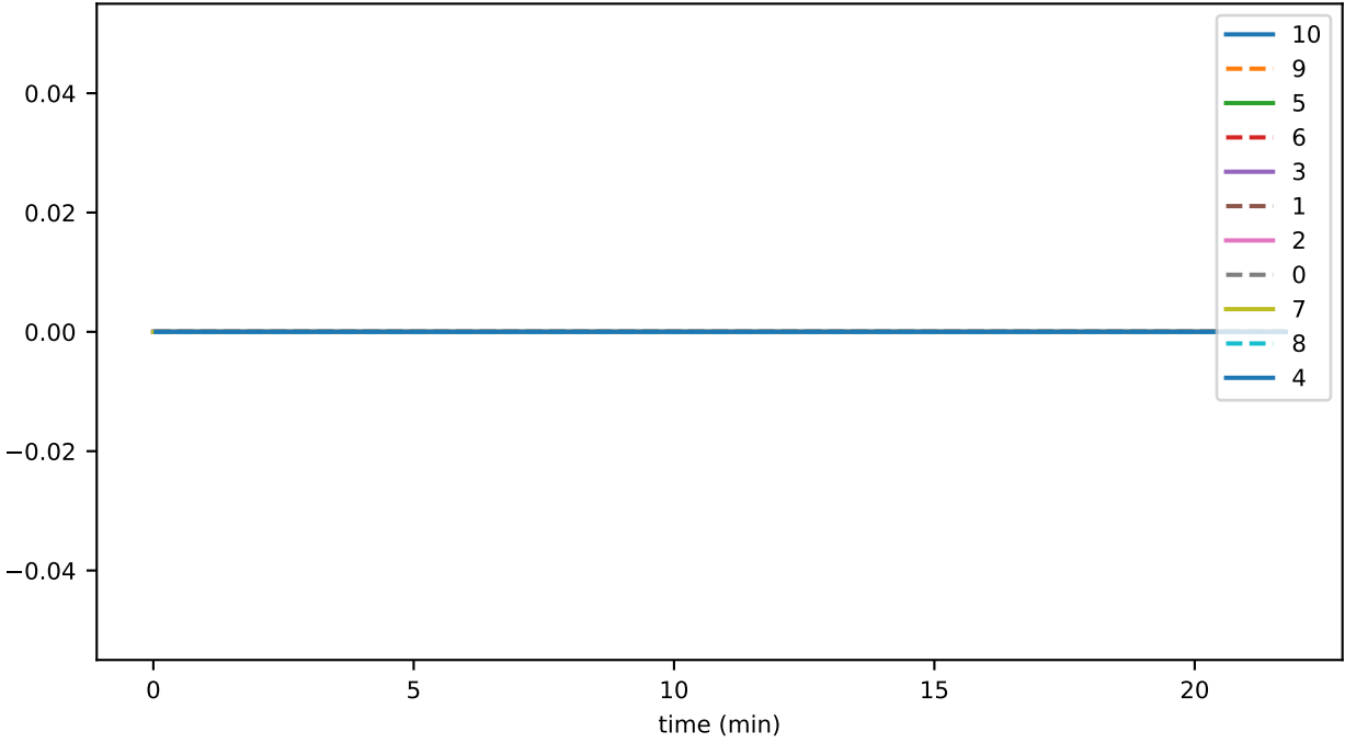
ds_compactions_level_0_hashesSavedSpaceMb_accounts
