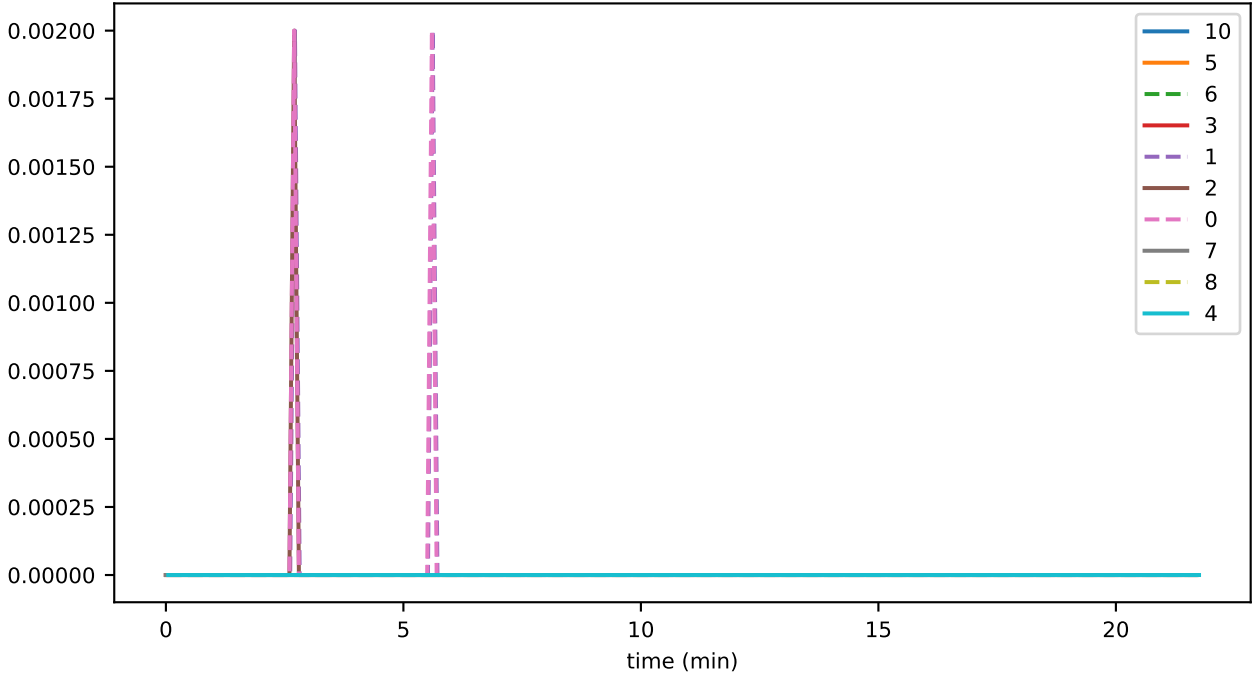
sync_phase_09_fraction_SELF_FALLEN_BEHIND
