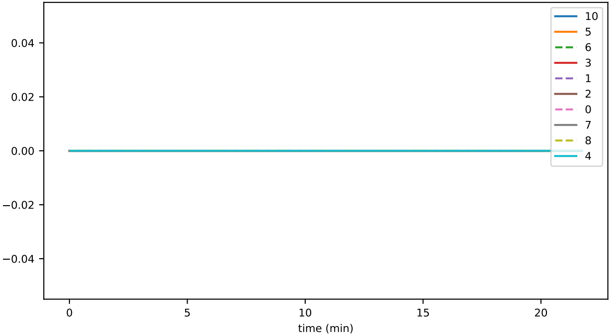
sync_phase_09_fraction_SELF_FALLEN_BEHIND
