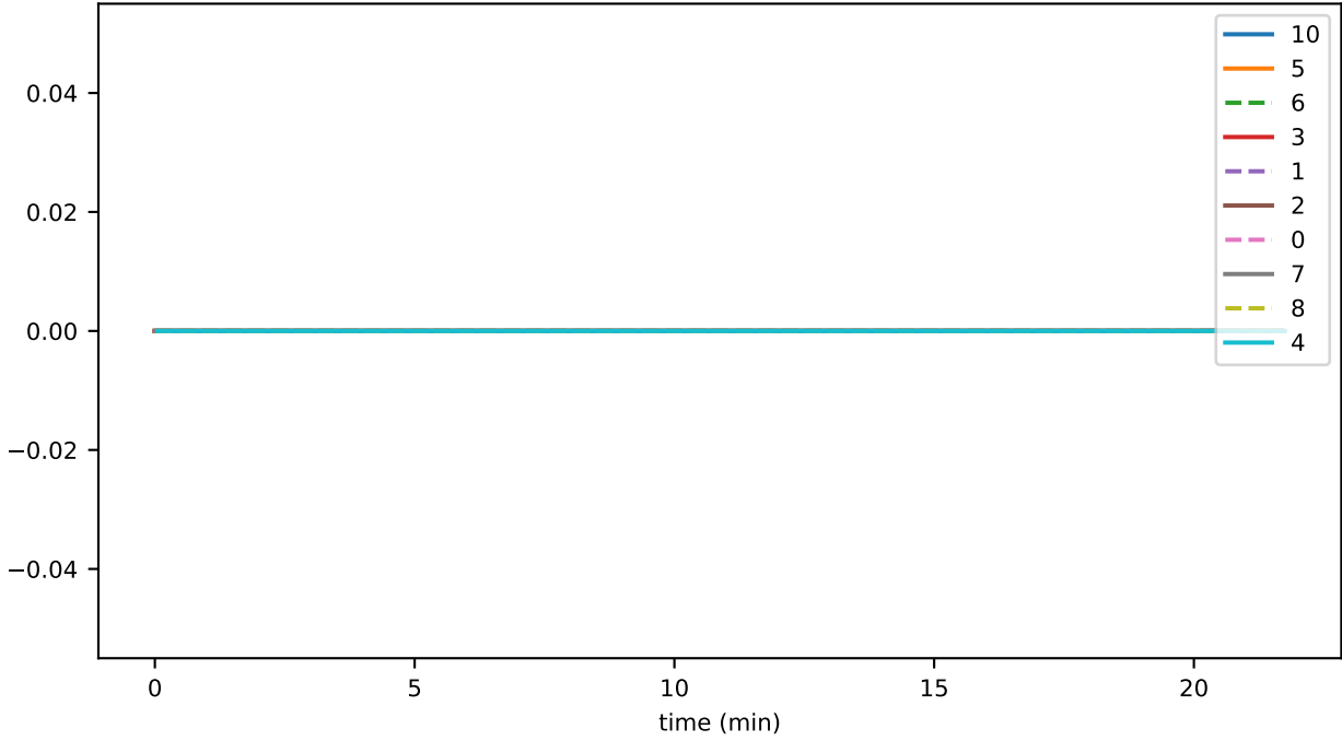
sync_phase_09_fraction_SENDING_EVENTS
