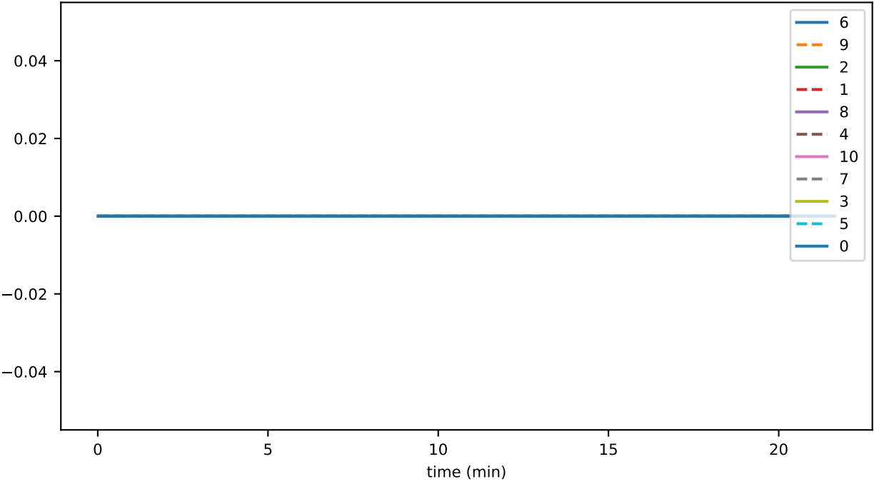
ds_compactions_level_0_hashesSavedSpaceMb_accounts
