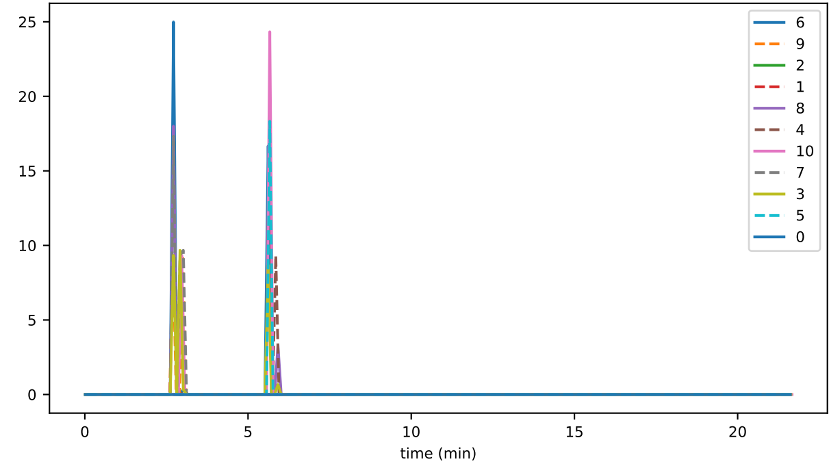
ds_compactions_level_0_hashesSavedSpaceMb_accounts
