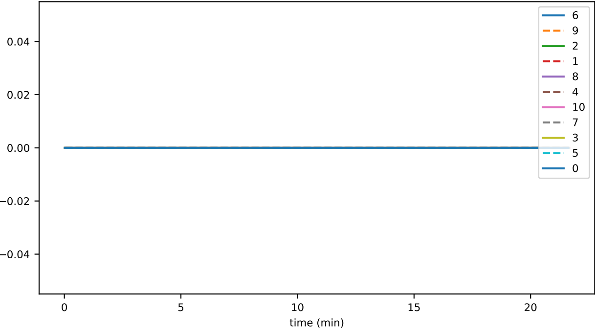
ds_compactions_level_0_hashesTimeMs_accounts
