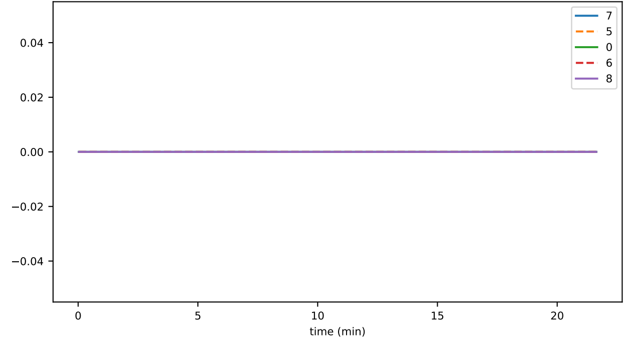
sync_phase_09_fraction_SENDING_EVENTS
