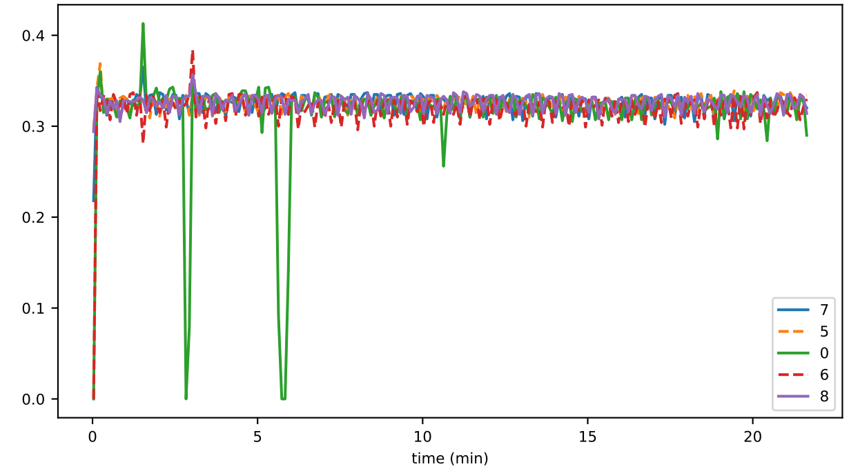
sync_phase_09_fraction_SENDING_EVENTS
