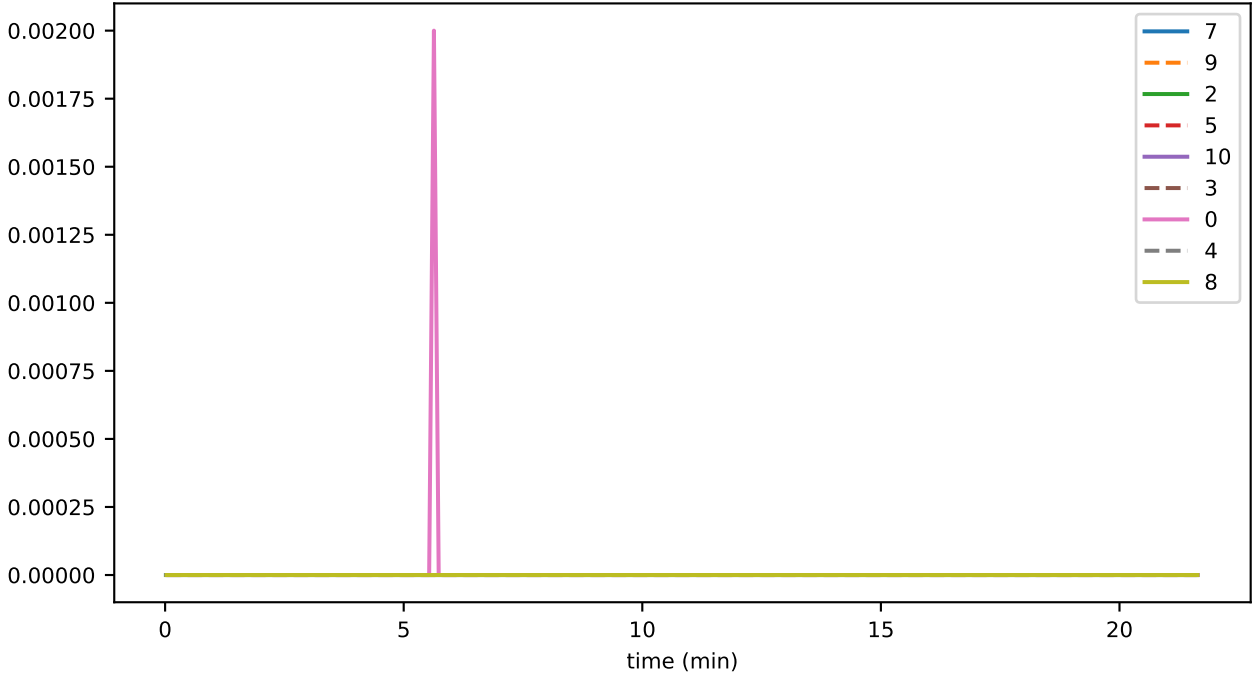
sync_phase_06_fraction_SELF_FALLEN_BEHIND
