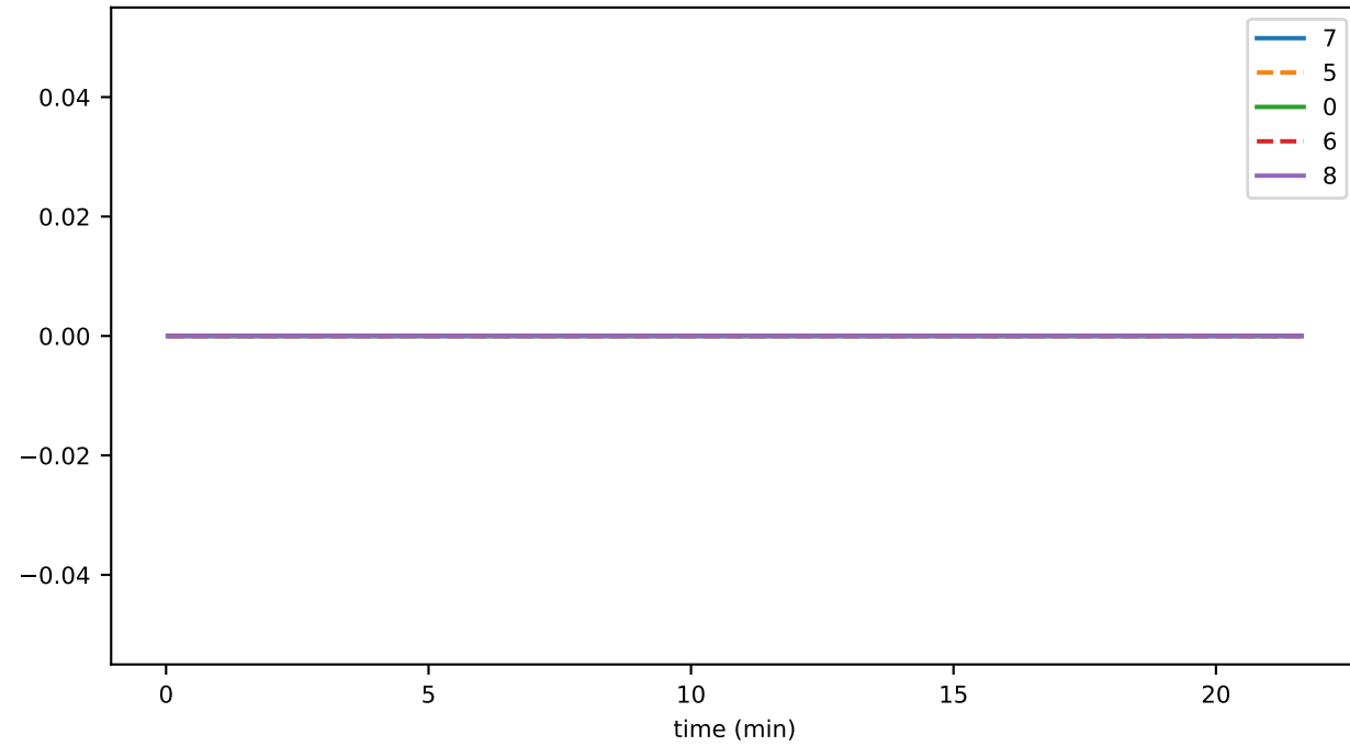
sync_phase_09_fraction_SELF_FALLEN_BEHIND
