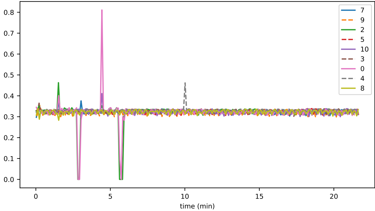
sync_phase_06_fraction_SENDING_EVENTS
