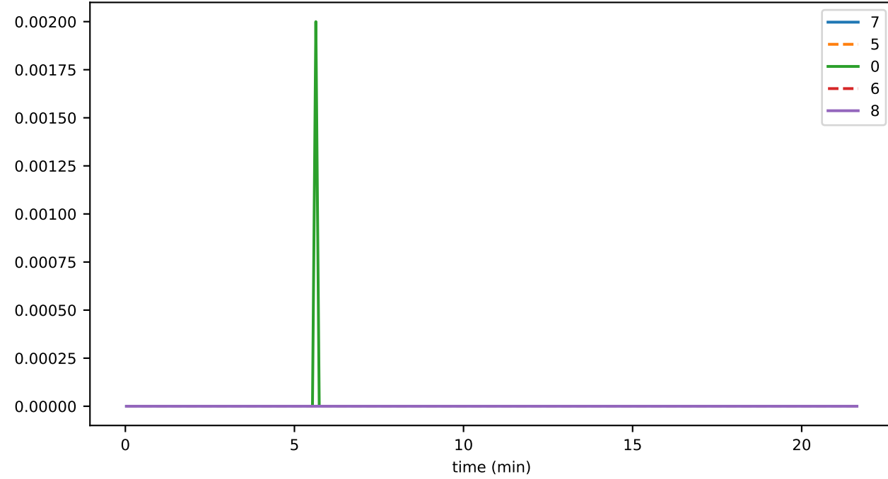
sync_phase_09_fraction_SELF_FALLEN_BEHIND
