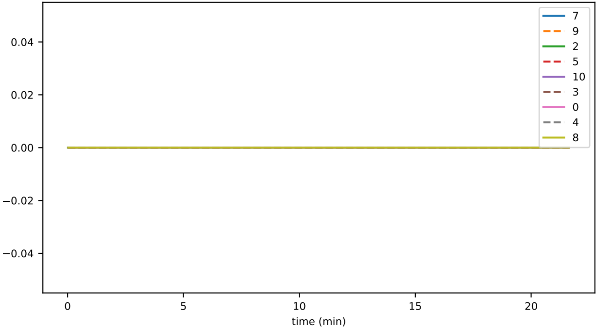
sync_phase_06_fraction_SELF_FALLEN_BEHIND
