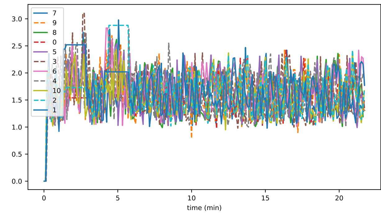
witnessesSeen
