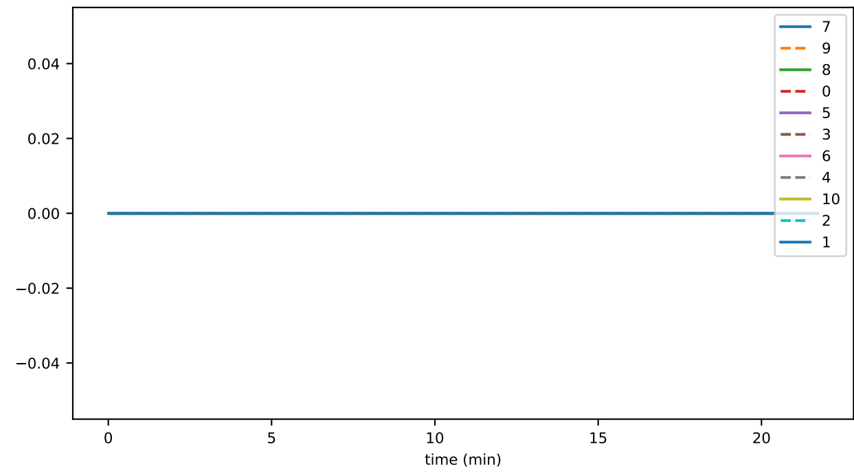
witnessesSeen
