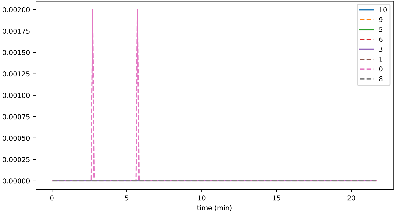
sync_phase_07_fraction_SELF_FALLEN_BEHIND
