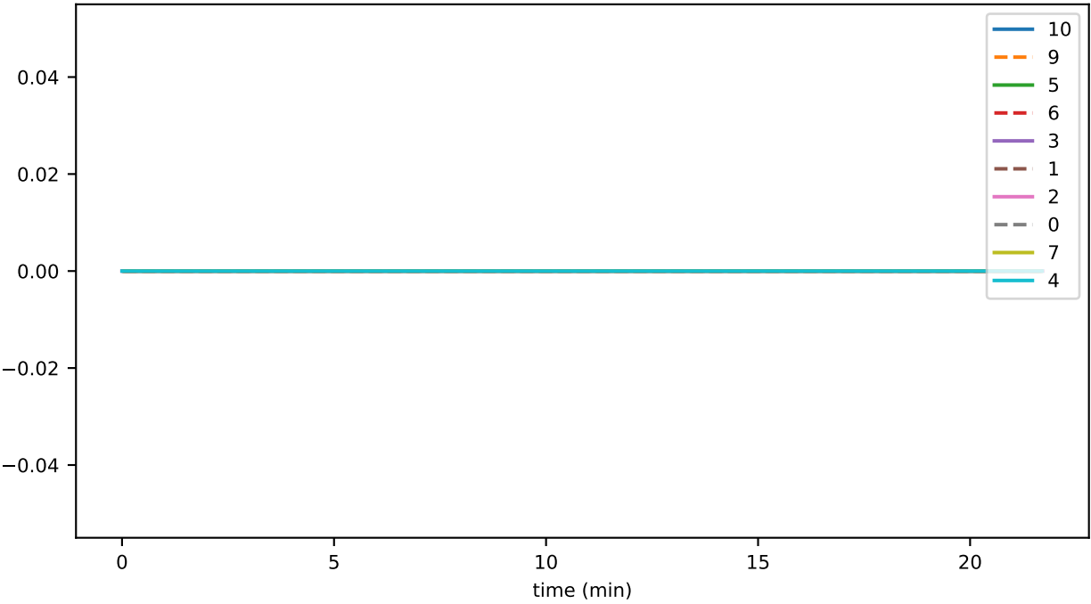
sync_phase_08_fraction_SELF_FALLEN_BEHIND
