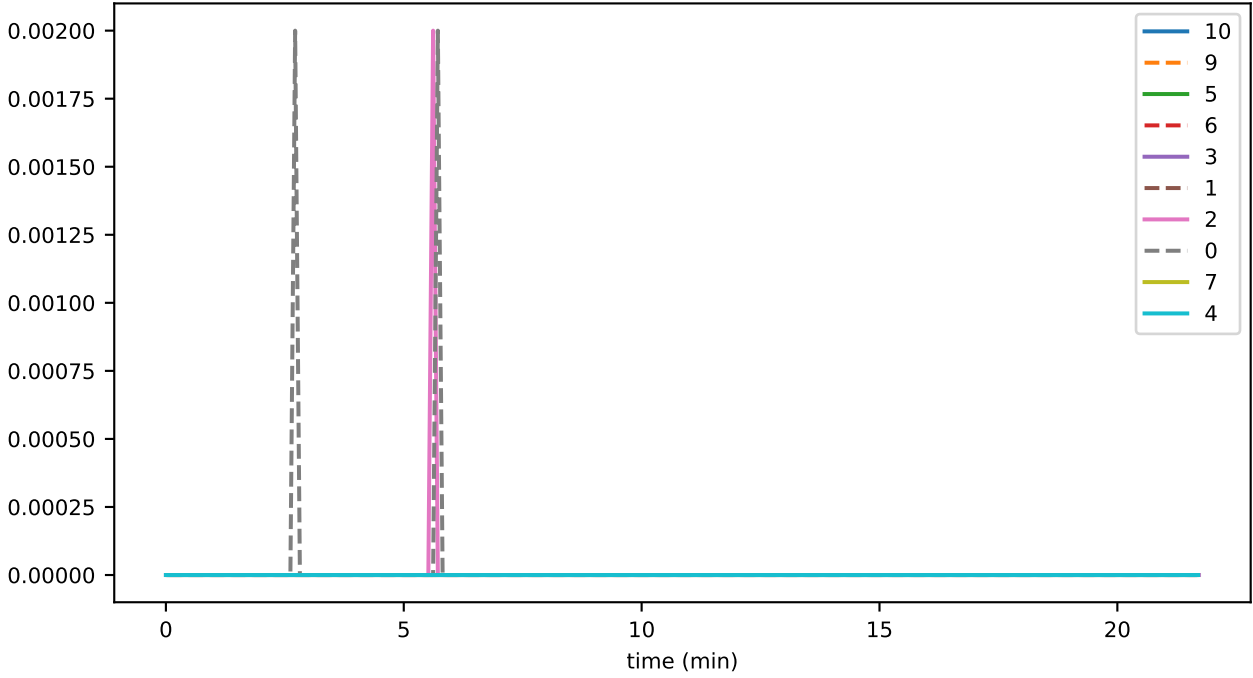
sync_phase_08_fraction_SELF_FALLEN_BEHIND
