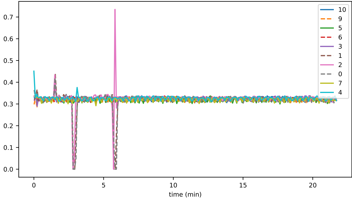
sync_phase_08_fraction_SENDING_EVENTS
