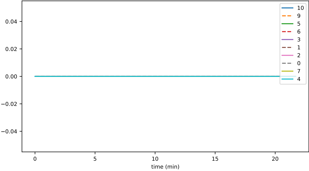
sync_phase_08_fraction_SENDING_EVENTS
