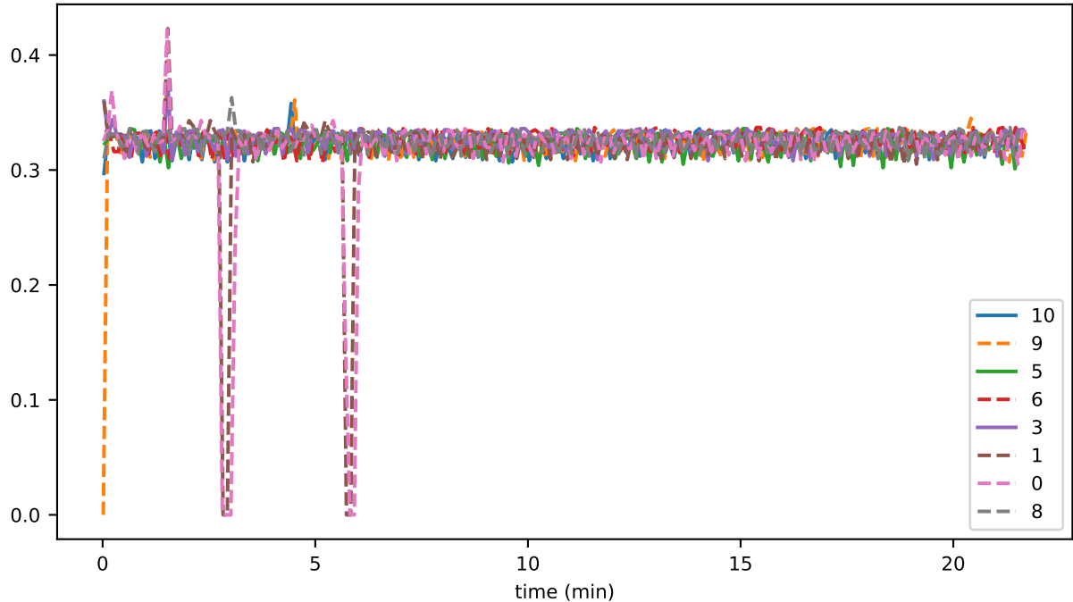
sync_phase_07_fraction_SENDING_EVENTS
