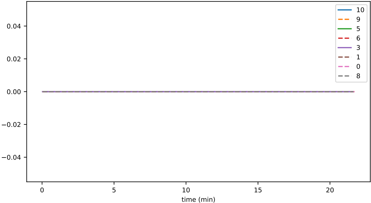
sync_phase_07_fraction_SELF_FALLEN_BEHIND
