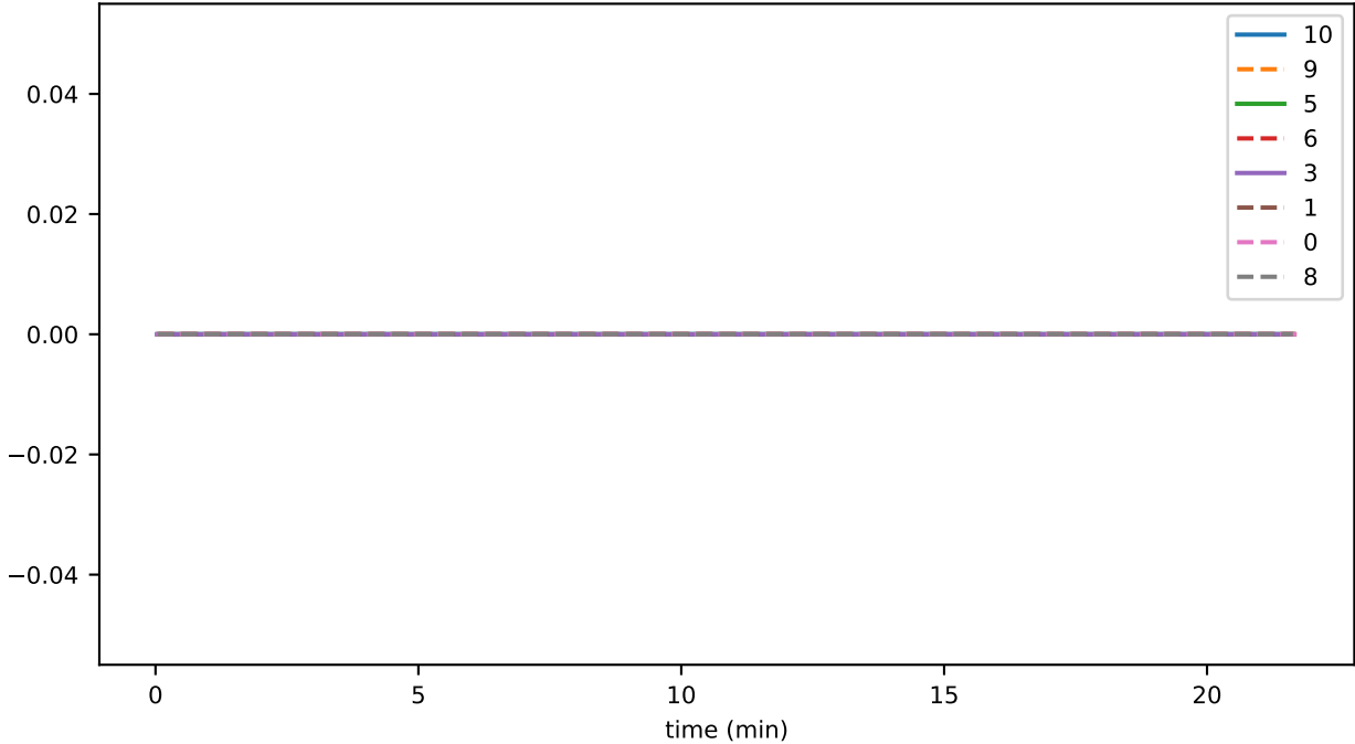
sync_phase_07_fraction_SENDING_EVENTS
