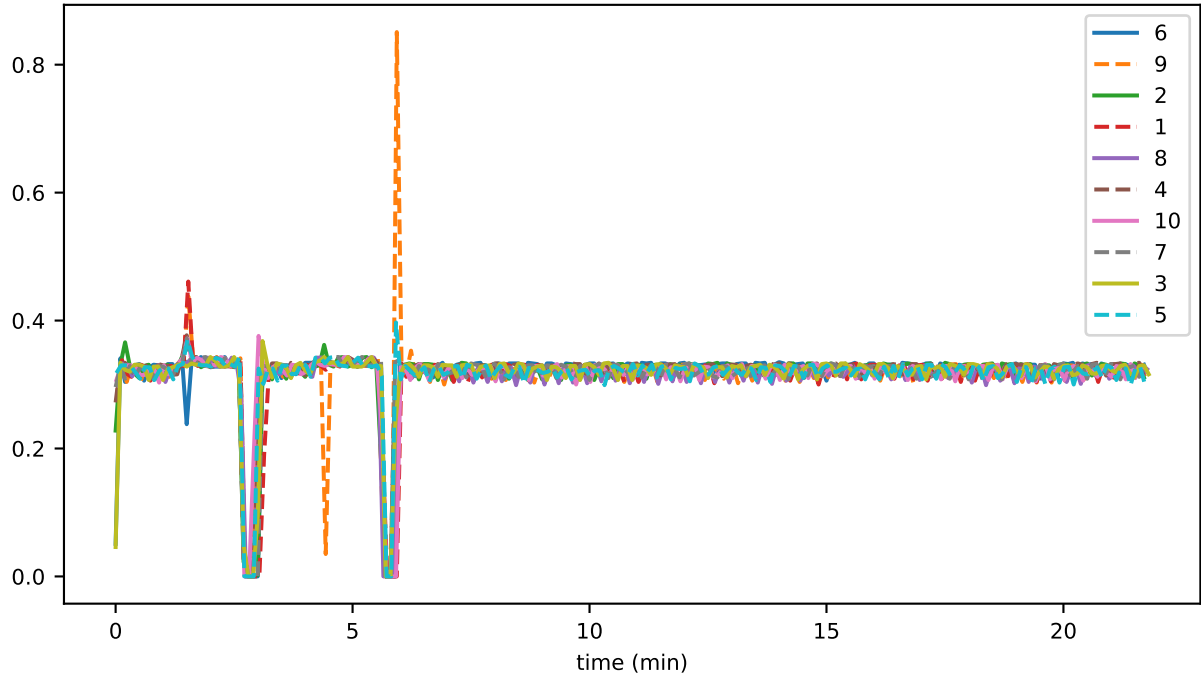
sync_phase_00_fraction_SENDING_EVENTS
