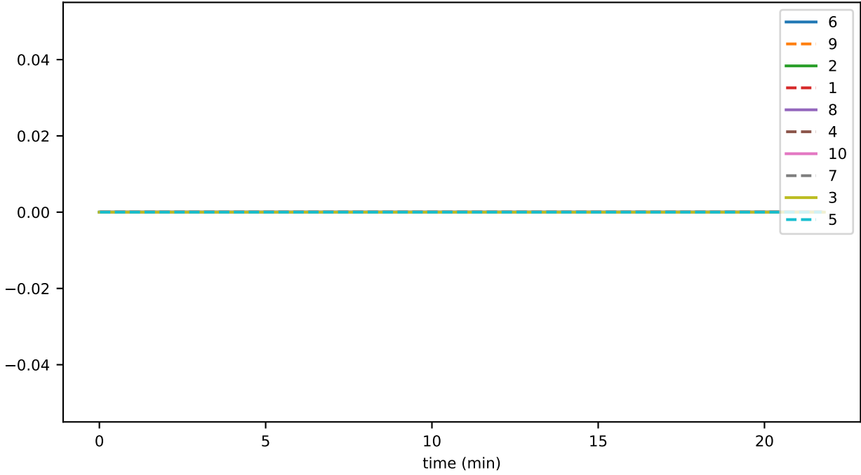
sync_phase_00_fraction_SENDING_EVENTS
