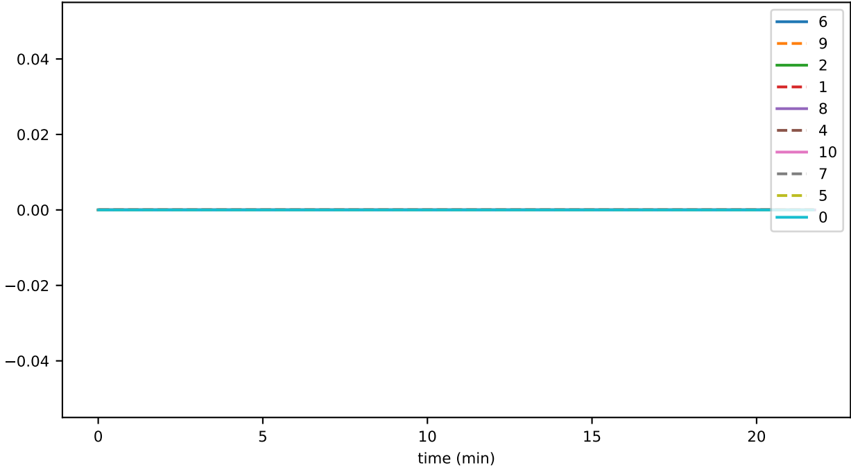
sync_phase_03_fraction_SENDING_EVENTS
