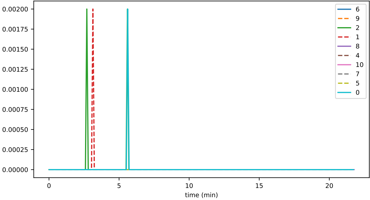
sync_phase_03_fraction_SELF_FALLEN_BEHIND
