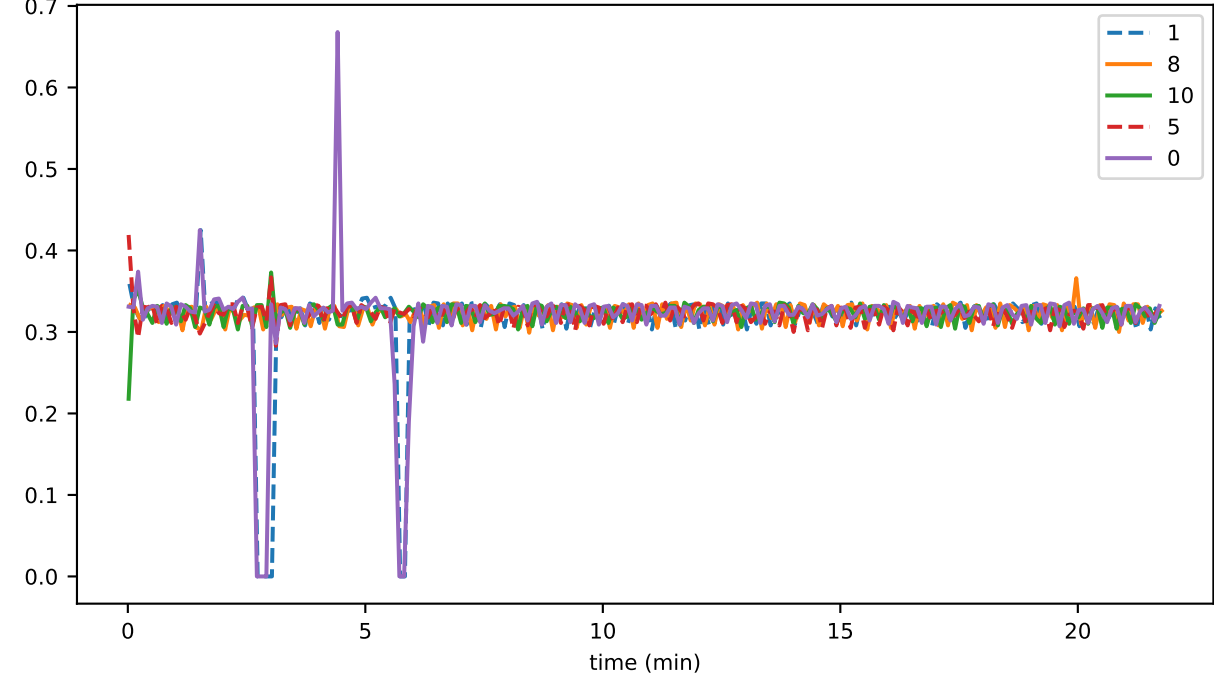
sync_phase_09_fraction_SENDING_EVENTS
