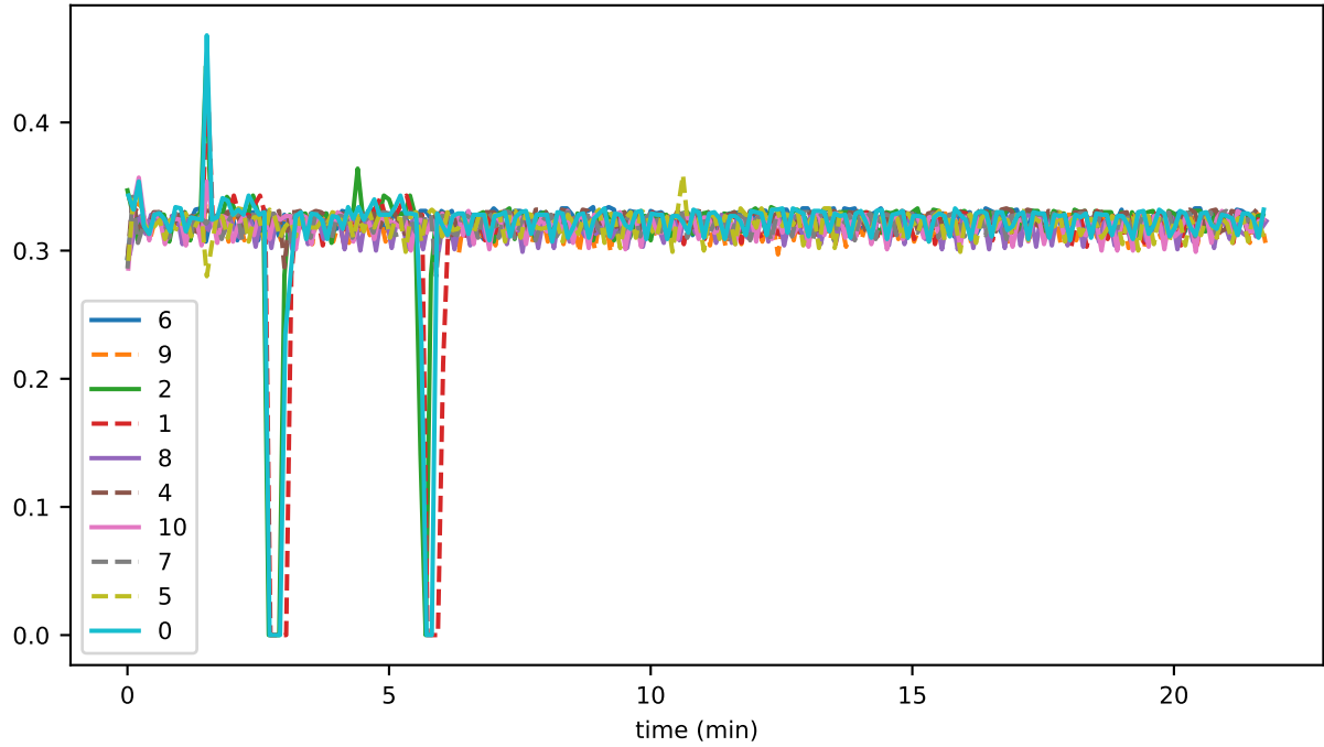
sync_phase_03_fraction_SENDING_EVENTS
