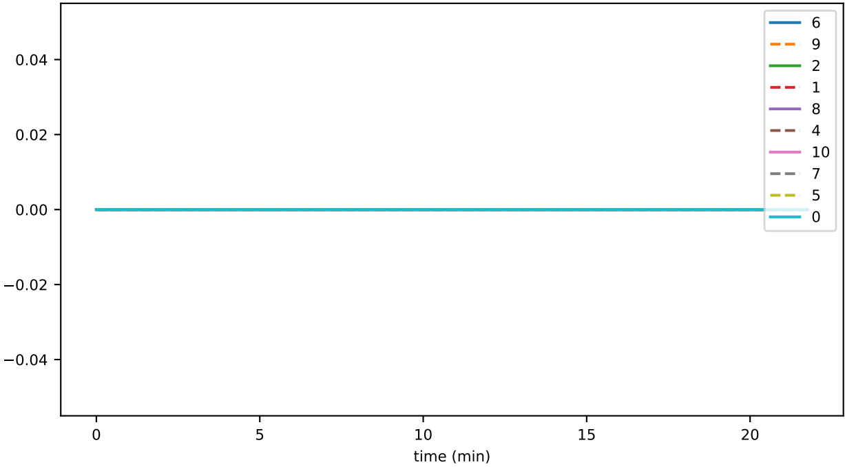
sync_phase_03_fraction_SELF_FALLEN_BEHIND
