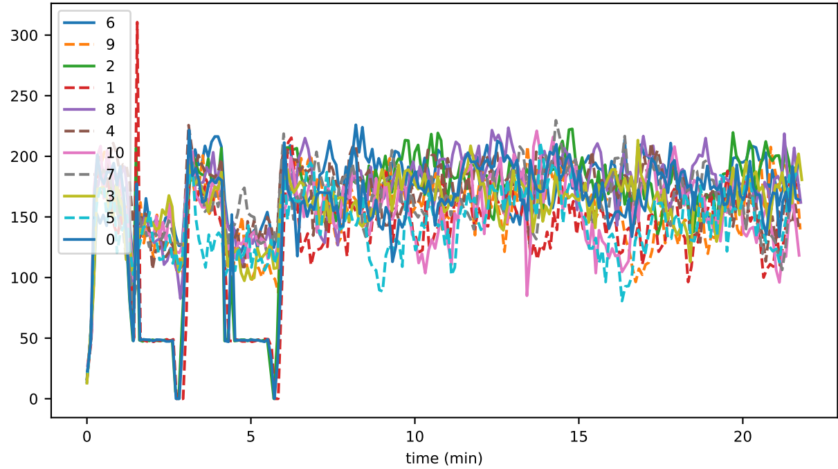
doNotSyncFallenBehind
