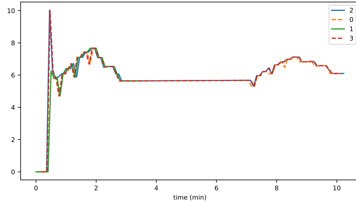
preconsensusEventFileOldestIdentifier
