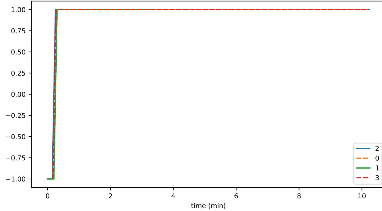
preconsensusEventFileOldestIdentifier
