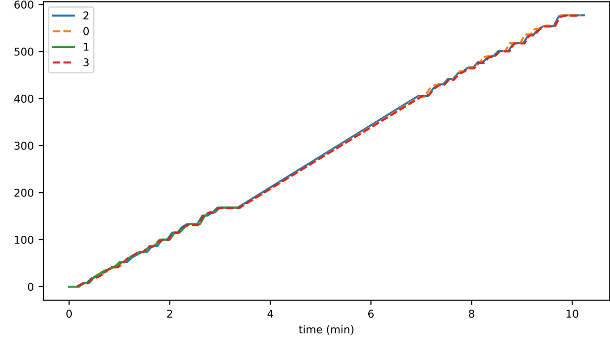
preconsensusEventFileOldestSeconds
