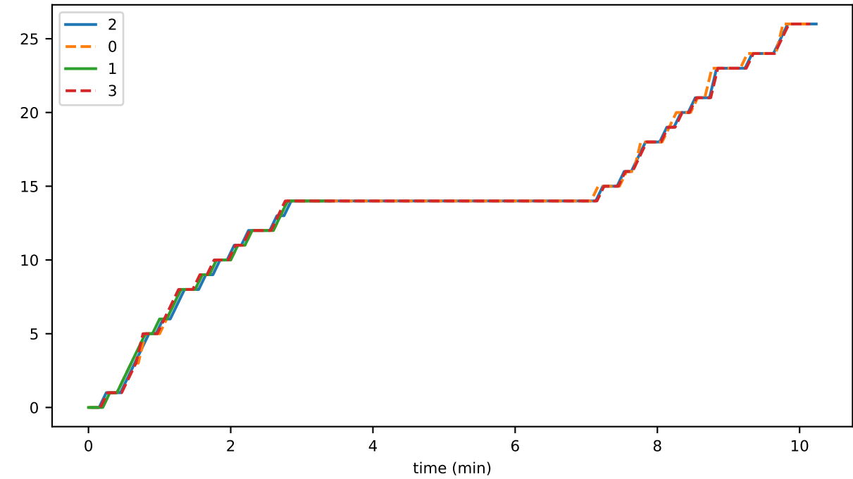
preconsensusEventFileOldestSeconds
