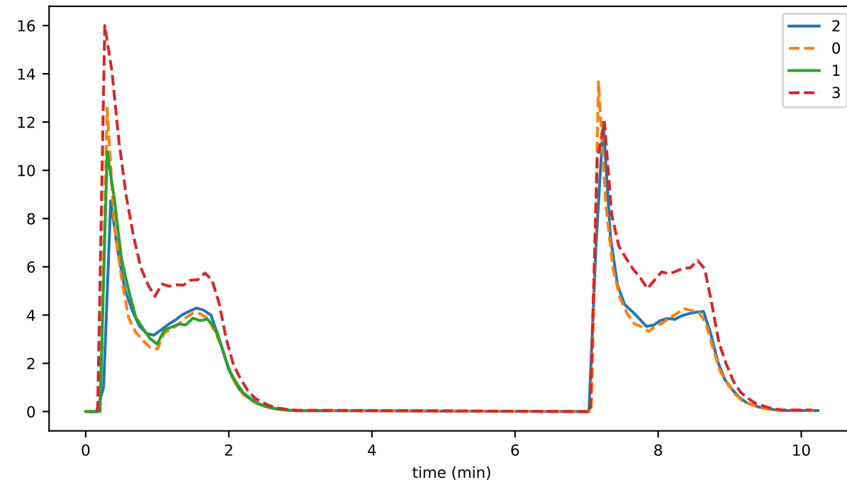
SigVal_per_sec
