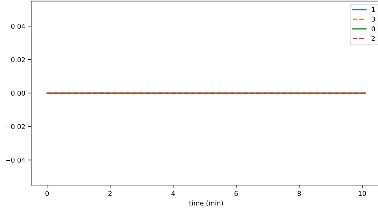
totalNeverSignedStates
