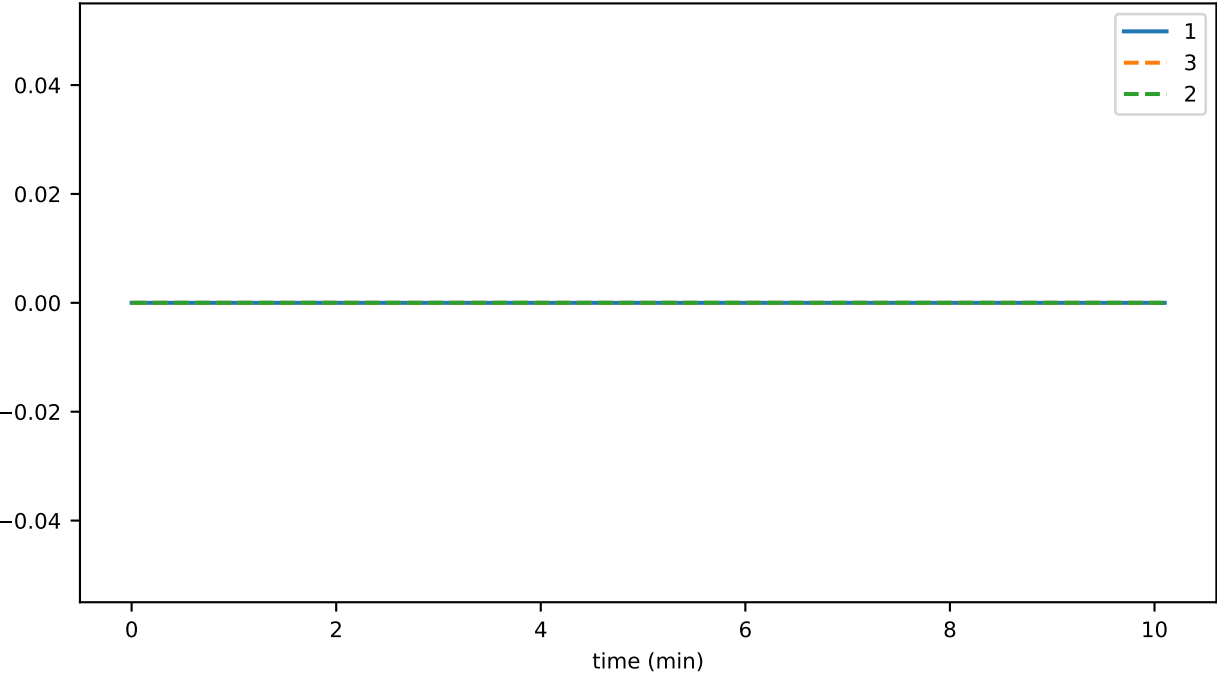
sync_phase_00_fraction_SENDING_EVENTS
