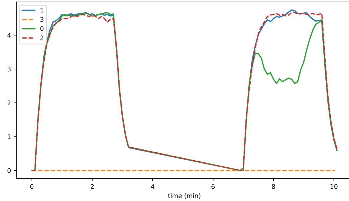
totalNeverSignedStates
