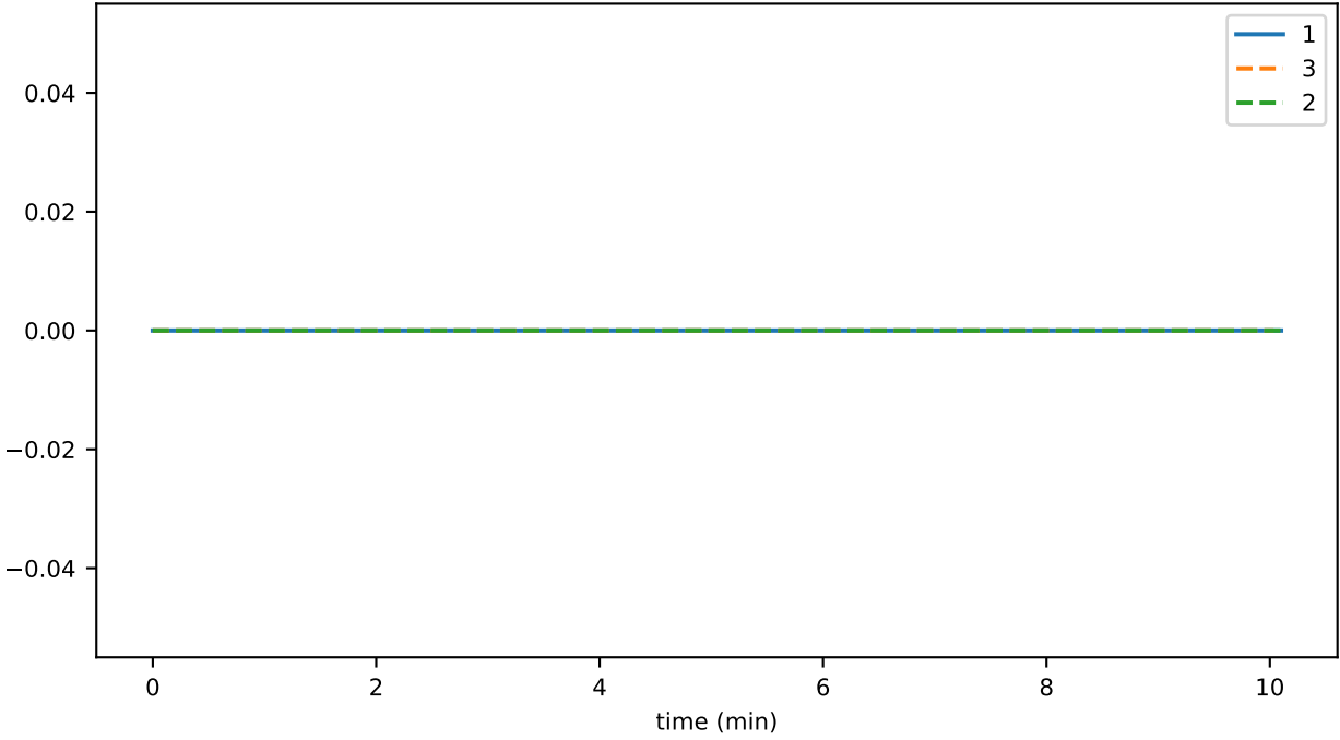
sync_phase_00_fraction_SELF_FALLEN_BEHIND
