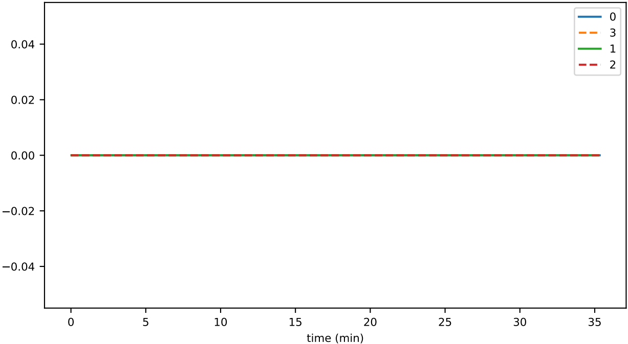
SmartContractService:SystemContractMethodCall_HSS_failed
